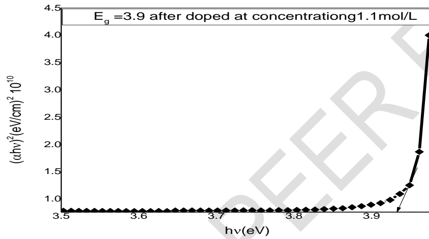
Fig. (8). (\alpha h\nu)^2 vs h\nu plot of Fe 2 O 3 doped TiO 2 thin films with concentration 1.1 mol/L
