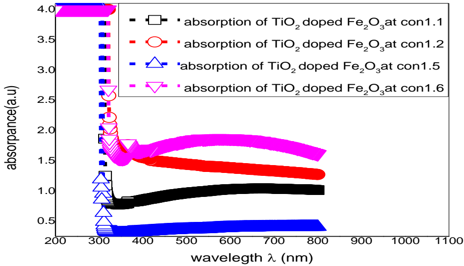
Fig.(3). Absorption vs wavelength plot of \text{Fe}_2\text{O}_3 doped \text{TiO}_2 thin films at different concentration (1.1, 1.2, 1.5 and 1.6 mol/L)
