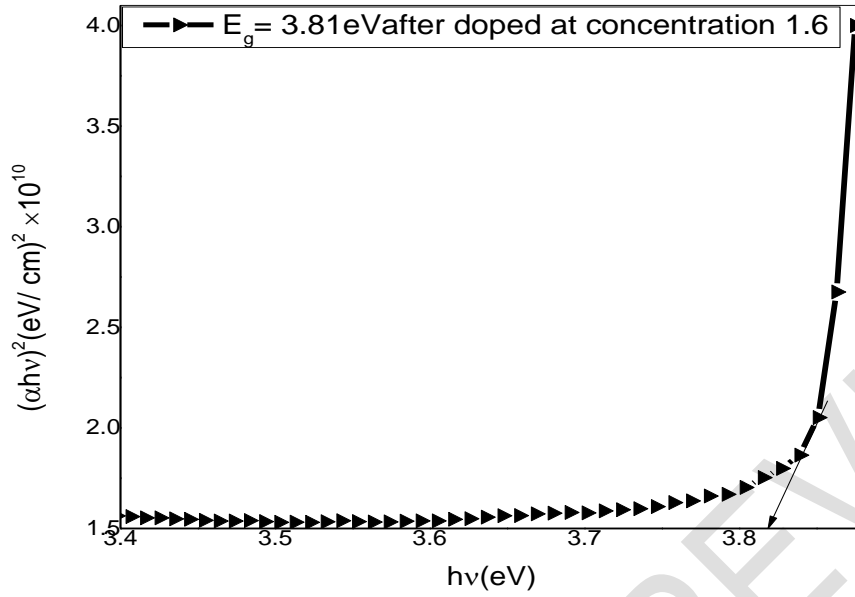
Fig. (11). (\alpha hv)^2 vs (hv) plot of Fe_2O_3 doped TiO_2 thin films with concentration 1.6mol/L
