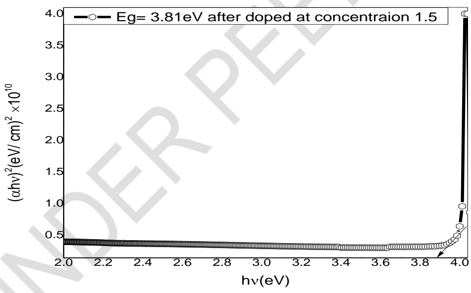
Fig (10) (\alpha hv)^2 vs (hv) plot of Fe_2O_3 doped TiO_2 thin films with concentration 1.5mol/L
