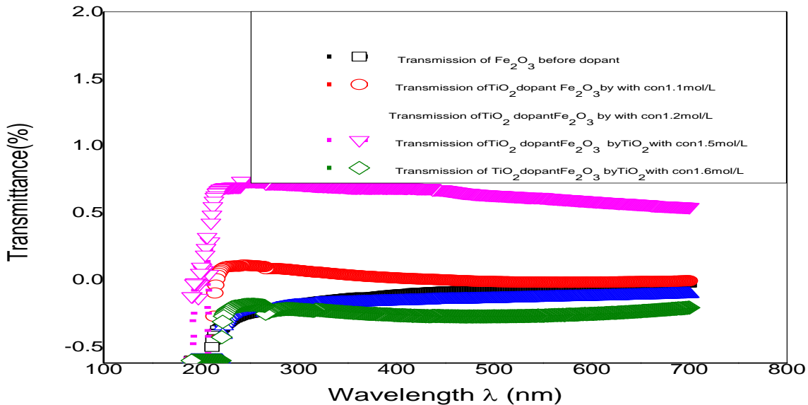
Fig. (4). Transmission vs wavelength plot of pure \text{Fe}_2\text{O}_3 and after doped \text{TiO}_2 thin films at different concentration (1.1, 1.2, 1.5 and 1.6 mol/L)
