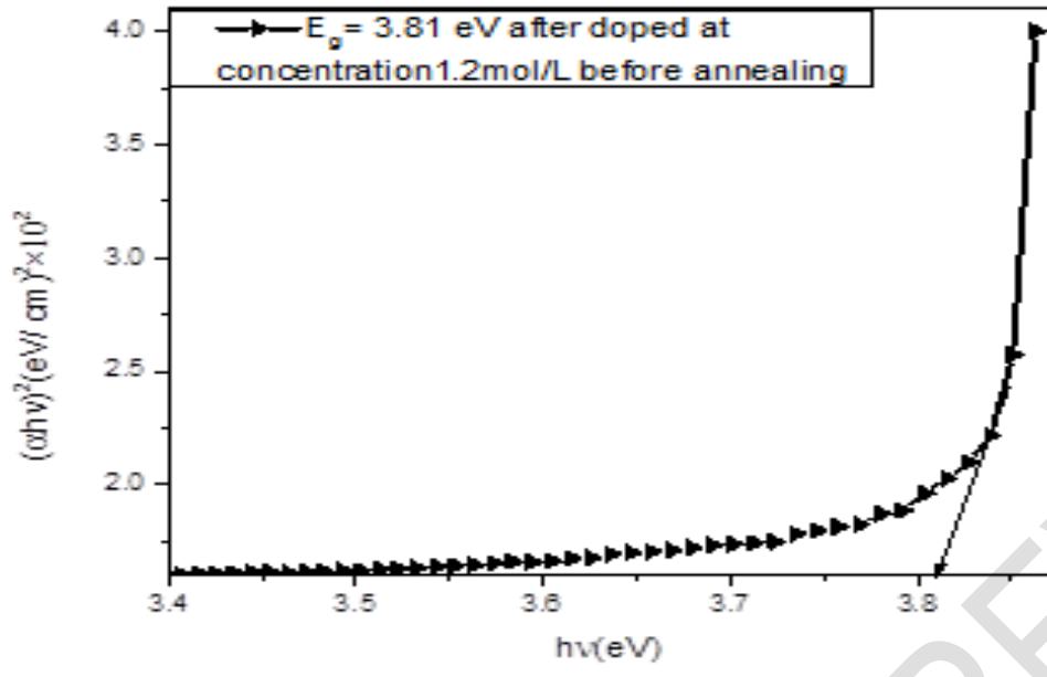
Fig (9) (\alpha hv)^2 vs (hv) plot of Fe_2O_3 doped TiO_2 thin films with concentration 1.2mol/L
