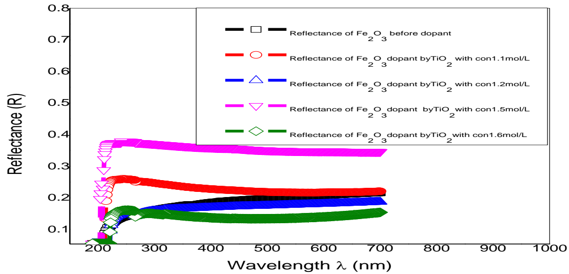
Fig.(5). Reflectance vs wavelength plot of \text{Fe}_2\text{O}_3 before and after doped \text{TiO}_2 thin films at different concentration (1.1, 1.2, 1.5 and 1.6mol/L)
