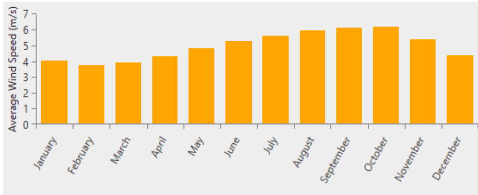
Figure 4: Monthly average wind speed in Dwangwa
