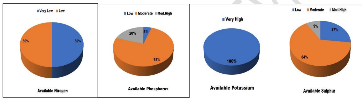
Fig 2: Categorization of soil available N, P, K, S from Washim road farm
