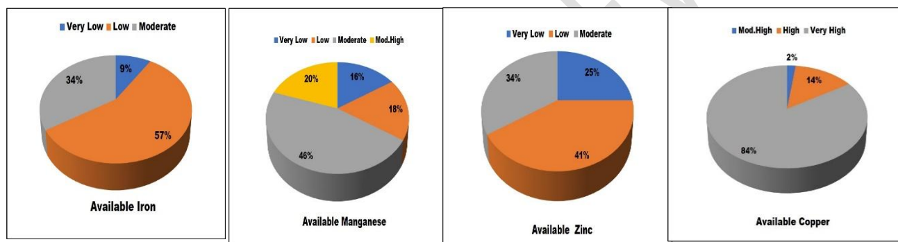
Fig 3: Categorization of soil available Fe, Mn, Zn, Cu from Washim road farm
