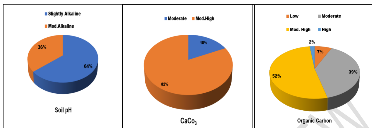
Fig 1: Categorization of soil pH, CaCO 3 , Organic Carbon from Washim road farm
