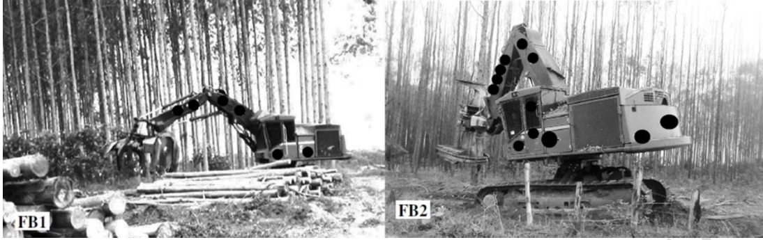
FIG. 1 Crawler Feller-buncher without leveling device – FB1; Crawler Feller-buncher with leveling device – FB2
