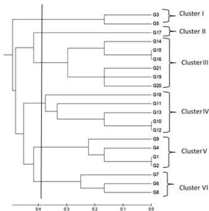
Fig. 2. UPGMA dendrogram based on genetic distance summarizing of 21 rice genotypes according to SSR analysis. Cophenetic Correlation Coefficient (CP) value was 0.50.
