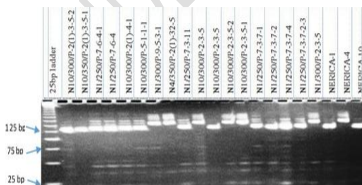
Fig. 1. Amplification profile of primer RM202 for 18 NERICA mutant lines along with their 3 parents.
