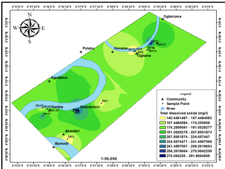
Figure 3a: Spatial distribution of groundwater
