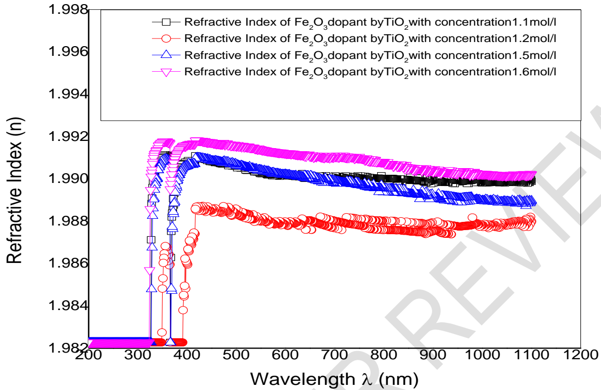
Fig.12. Refractive index vs. wavelength plot of Fe 2 O 3 after doped TiO 2 thin films different at the concentration (1.1, 1.2, 1.5 and 1.6mol/L)
