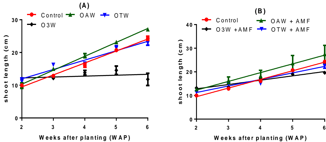
Figure 3.1. (A) Shows shoot length responses of non-mycorrhizal A. esculentus under drought stress (B) shows improved growth of A. esculentus under drought stress as a result of AMF inoculation. Under extreme stress condition, it could be observed that AMF inoculation stimulated growth close to that of the control when compared to its uninoculated counterpart.
