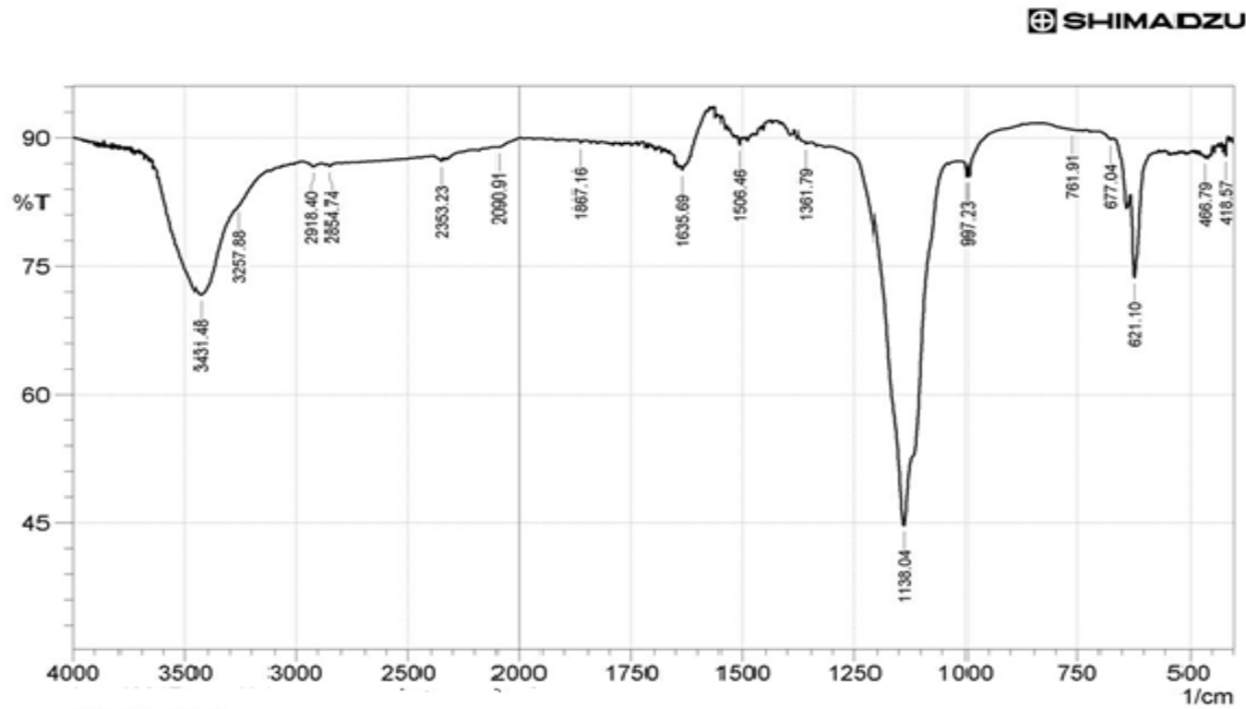
Fig. 1. FTIR spectrum of ZnS powder
