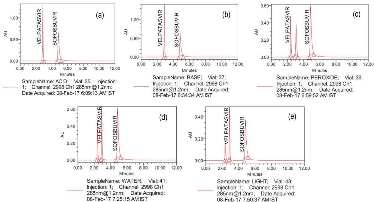
240 Figure 8: Degradation Chromatogram working standard solutions of valpatasvir & sofosbuvir 241 after (a) Acid hydrolysis (0.1 N HCl, refluxed for 1 H at 80°C) (b) Alkali (0.1 N NaOH refluxed 242 for 4H at 80°C) and (c) Oxidative degradation (3% H 2 O 2 Stored at room temperature) (d) Water 243 degradation (e) UV light degradation (near UV \geq 200 for 10 days).
