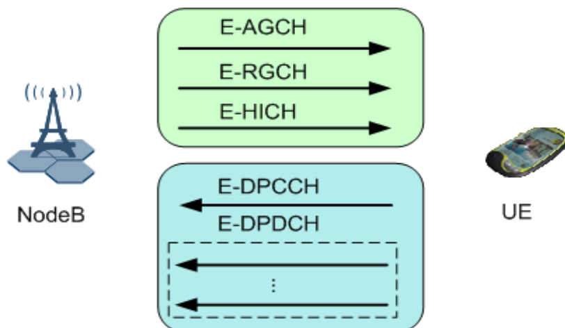
Figure 1: HSUPA Physical Channels
