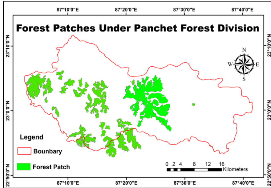
Fig-2: Forest patches from landuse/land cover map of PFD. IRS LISS-III P6 image 2016
