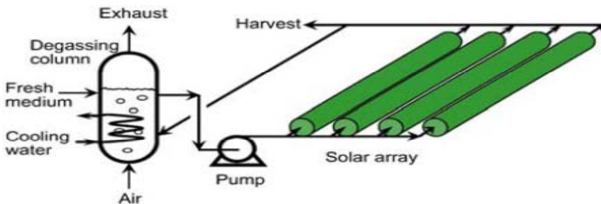
Figure 1: A diagrammatic representation of algae production using tubular photobioreactors
