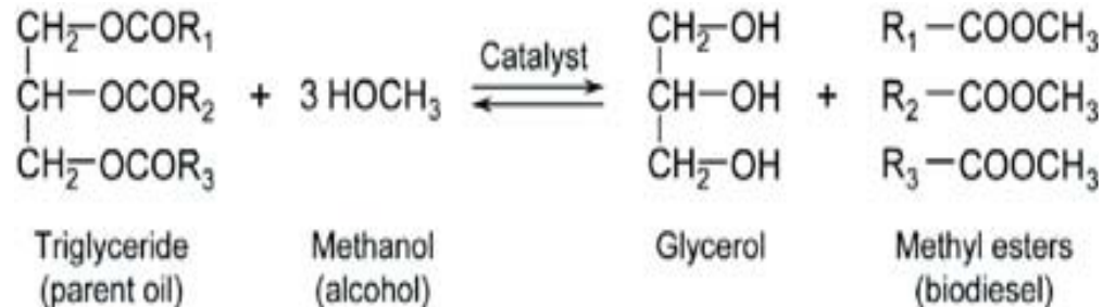
Figure 3: Transesterification of oil to biodiesel (R d1–3 are hydrocarbon groups).
