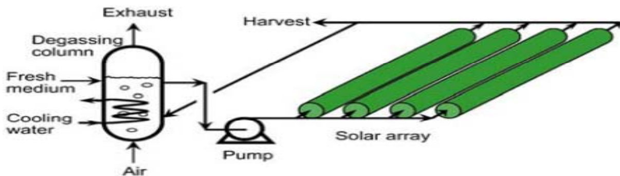
Figure 1: A diagrammatic representation of algae production using tubular photobioreactors
