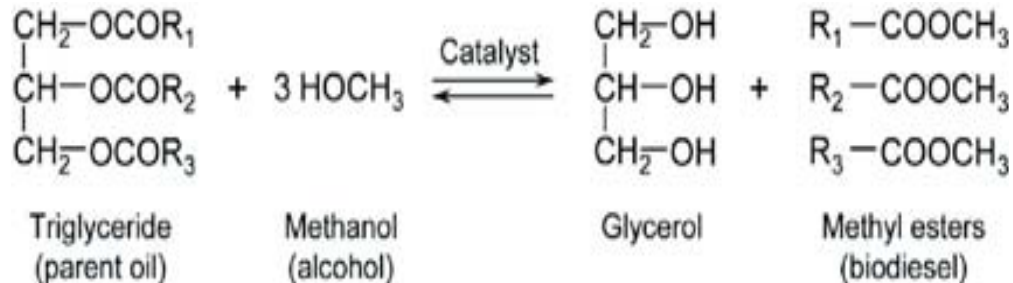
Figure 4: Transesterification of oil to biodiesel (R d1–3 are hydrocarbon groups).
