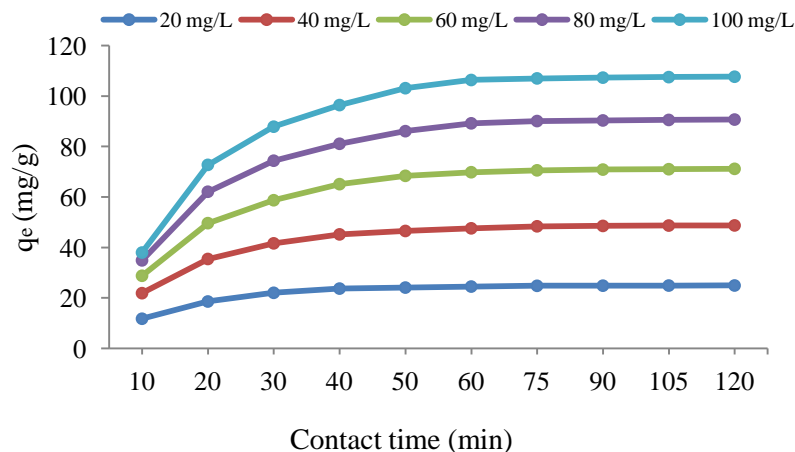
Fig. 3. Effect of contact time and initial concentration on SMZ adsorption (pH =7, Adsorbent dosage 0.8 g/L, mixing rate 150 rpm, temp= 25 \pm 2^\circ\text{C} )
