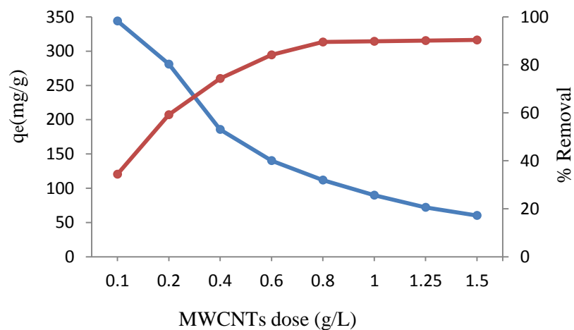
Fig. 2. Effect of adsorbent dosage on SMZ adsorption ( C_0 = 100 mg/L, time = 75 min, pH = 7, temp= 25 \pm 2^\circ\text{C} and mixing rate 150 rpm)
