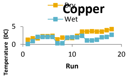
Fig. 6: Graph of Temperatures changes in Dry and Wet Copper against Number of run
