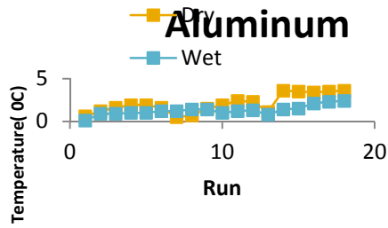
Fig. 5: Graph of Temperatures changes in Dry and Wet Aluminium against Number of run
