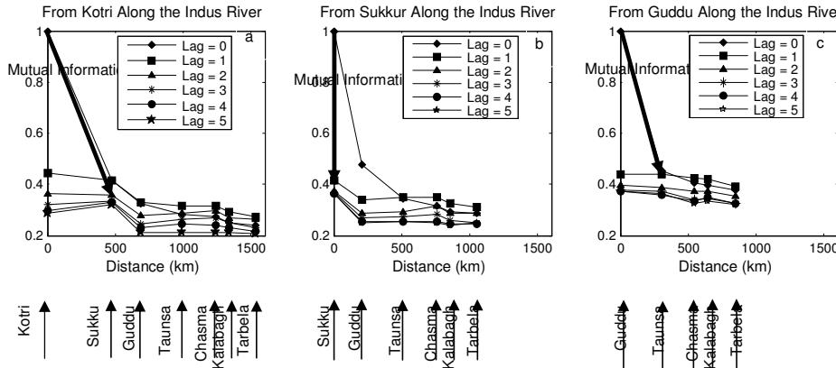
Fig. 3 The NR curve (Thick line) behaviour acquired from space-time MI analysis (obtained as the same procedure developed in Figs. 1 & 2), from lower three stations (a) Kotri, (b) Sukkur, and (c) Guddu with itself and with all its upstream station's along Indus River.
