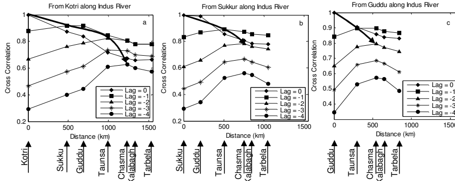
Fig. 2 The LR curve (Thick line) is prominently viewed over CROSS-CORRELATION value curves prominently (thin line) in space-time CROSS-CORRELATION analysis (method developed and transformed from Fig. 1.1), from lower three stations (a) Kotri, (b) Sukkur, and (c) Guddu with itself and with all its upstream station's along Indus River.
