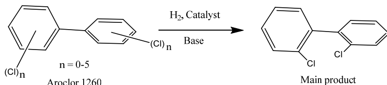
Scheme 1. Hydrodechlorination of Aroclor 1260.
