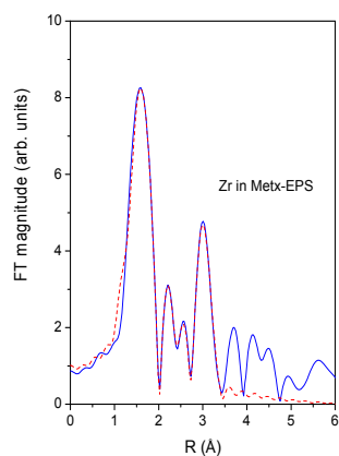
Fig. 5. Fourier transform magnitude of k3-weighted Zr K-edge EXAFS spectra of Zr in Met x -EPS sample, calculated in the k range 3–11 Å -1 and R range 1–3.4 Å. Experiment: solid line; best-fit EXAFS model of the nearest coordination shells: dashed line.
