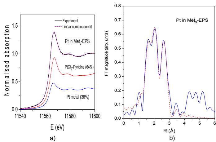
Fig. 3. a) Pt L3-edge XANES spectrum measured on the Pt in Metx-EPS sample: Black solid line: experiment; magenta dashed line: best-fit linear combination of XANES profiles of Pt fcc metal (36%), and cis-dichlorobis pyridine platinum reference compound (64%); b) Fourier transform magnitude of k 2 -weighted Pt L3-edge EXAFS spectra of Pt in Metx-EPS sample, calculated in the k range 3–12 Å -1 and R range 1–3.8 Å. Experiment: solid line; best-fit EXAFS model of the nearest coordination shells: dashed line.
