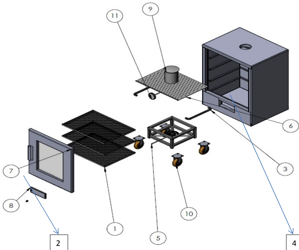
Fig. 1: Exploded View of the Gas oven
