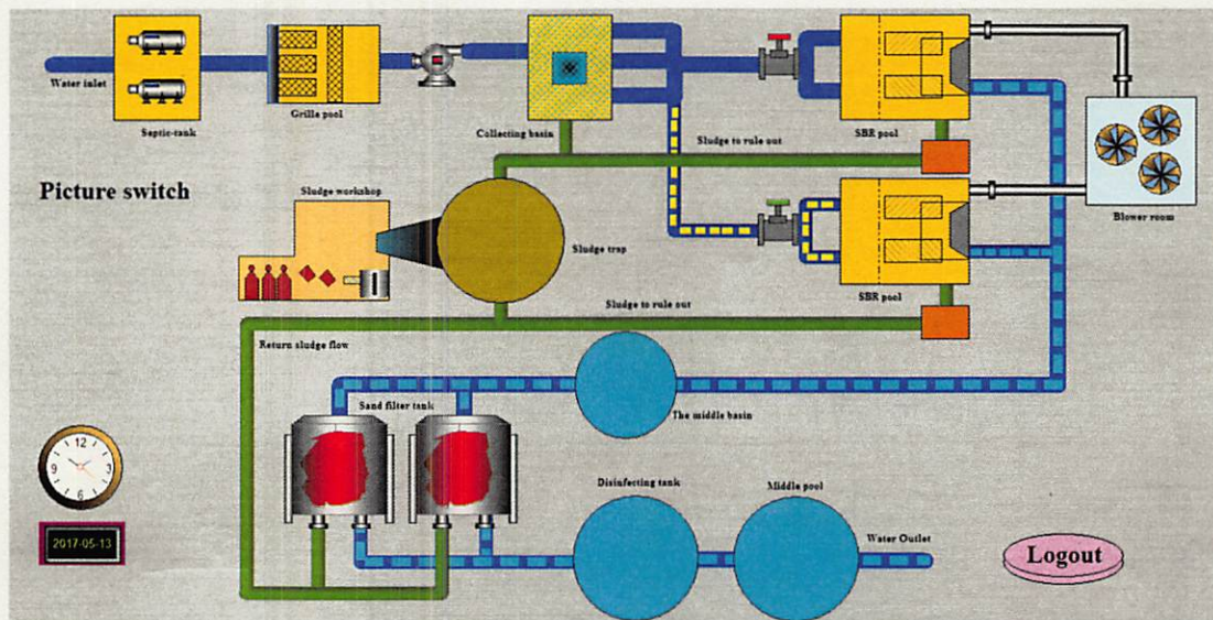
Fig.6 Main screen of the system
