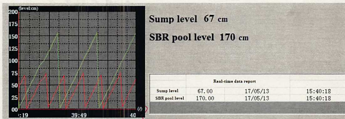
Fig.10 Real-time trend curve
