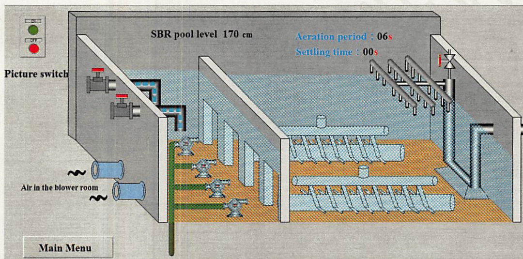
Fig.8 SBR pool
