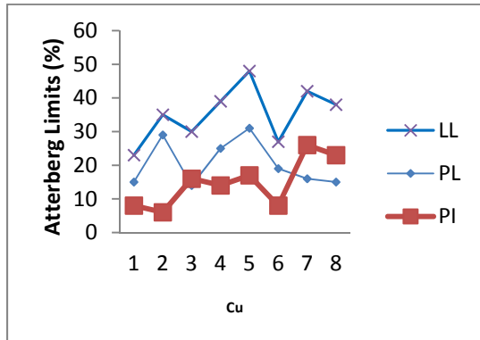
Figure 4: Relationship between Atterberg limits and coefficient of uniformity
