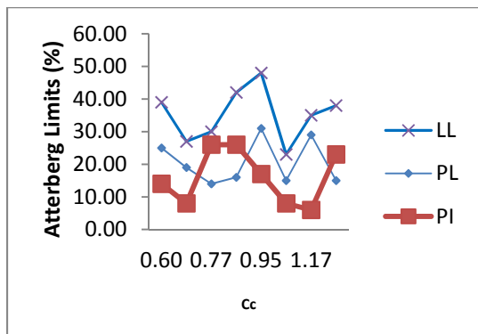
Figure 5: Relationship between Atterberg limits and coefficient of gradation
