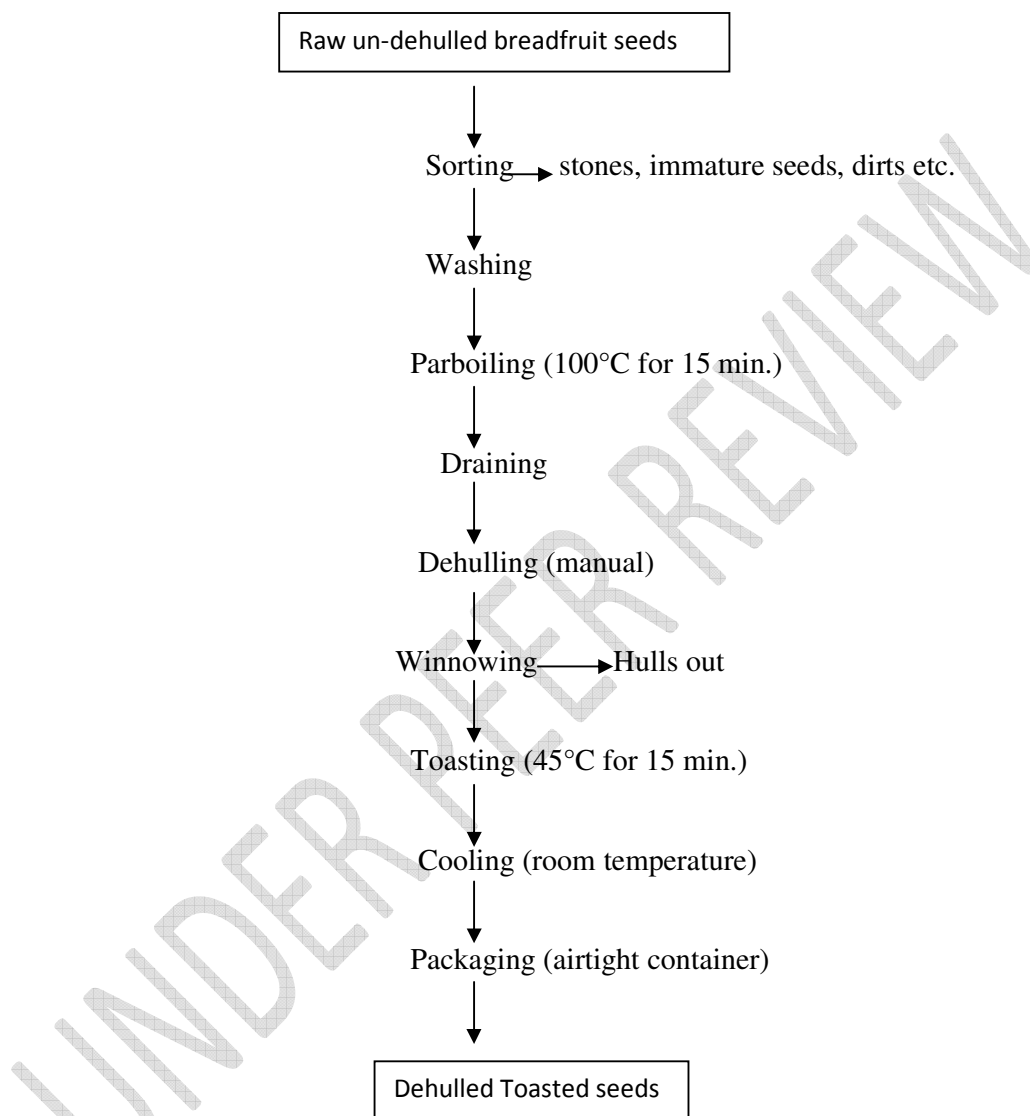
Figure 1: Flow chart for dehulled toasted breadfruit seeds
