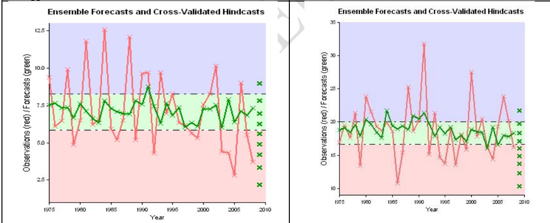
Fig. 14. Ensemble prediction of rainfall and Cross-Validated Hindcasts for rainy season at Barisal. Fig. 15. Ensemble prediction of rainfall and Cross-Validated Hindcasts for rainy season at Sylhet.
