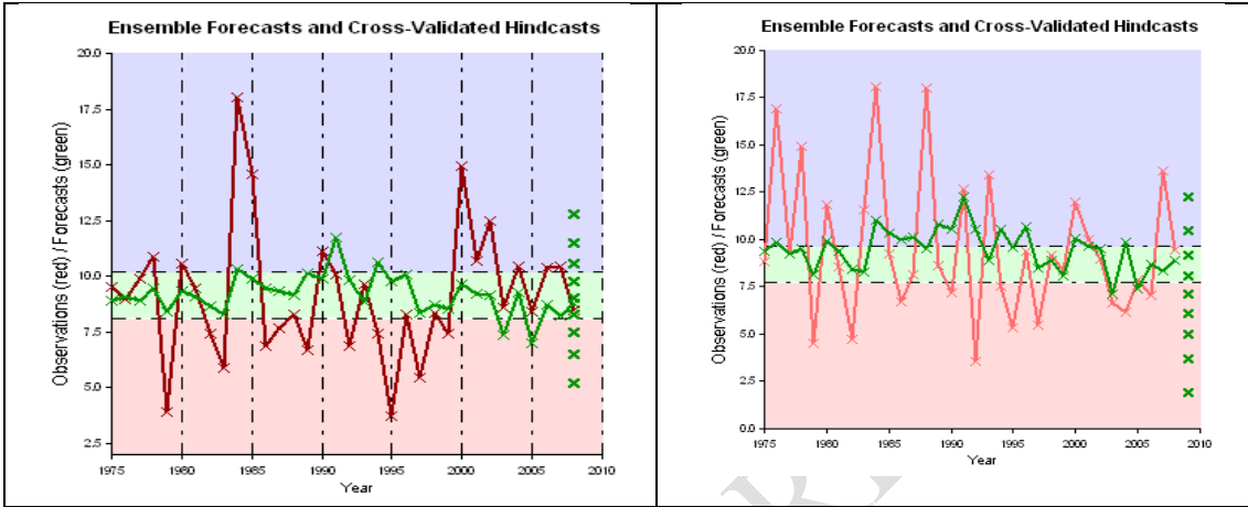
Fig. 12. Ensemble prediction of rainfall and Cross-Validated Hindcasts for rainy season at Rangpur. Fig. 13: Ensemble prediction of rainfall and Cross-Validated Hindcasts for rainy season at Dhaka.
