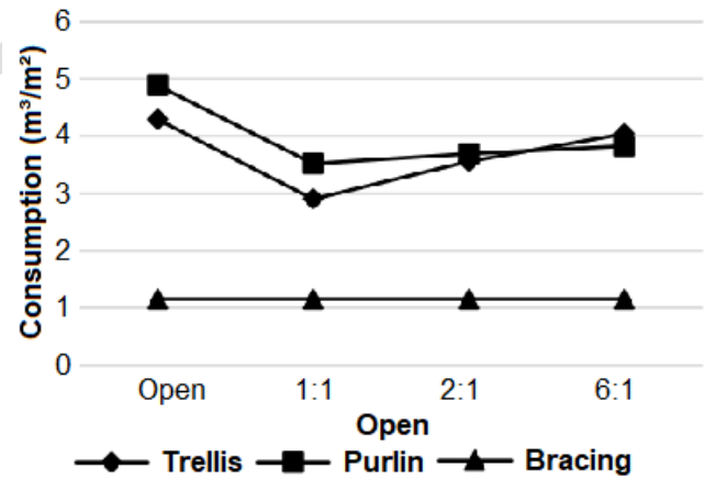
Figure 8 - Comparative consumption - 14 meters span.
