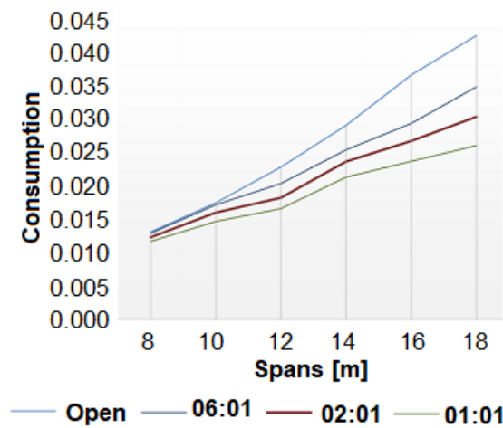
Figure 4 - Comparative consumption - all spans.
