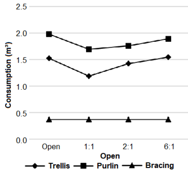
Figure 6 - Comparative consumption - 10 meters span.
