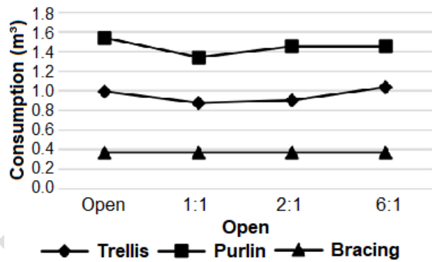
Figure 5 - Comparative consumption - 8 meters span.
