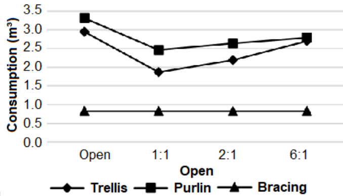
Figure 7 - Comparative consumption - 12 meters span.
