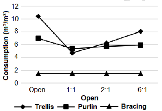
Figure 10 - Comparative consumption - 18 meters span.
