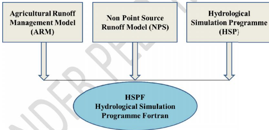
Fig2. Development of HSPF Model
