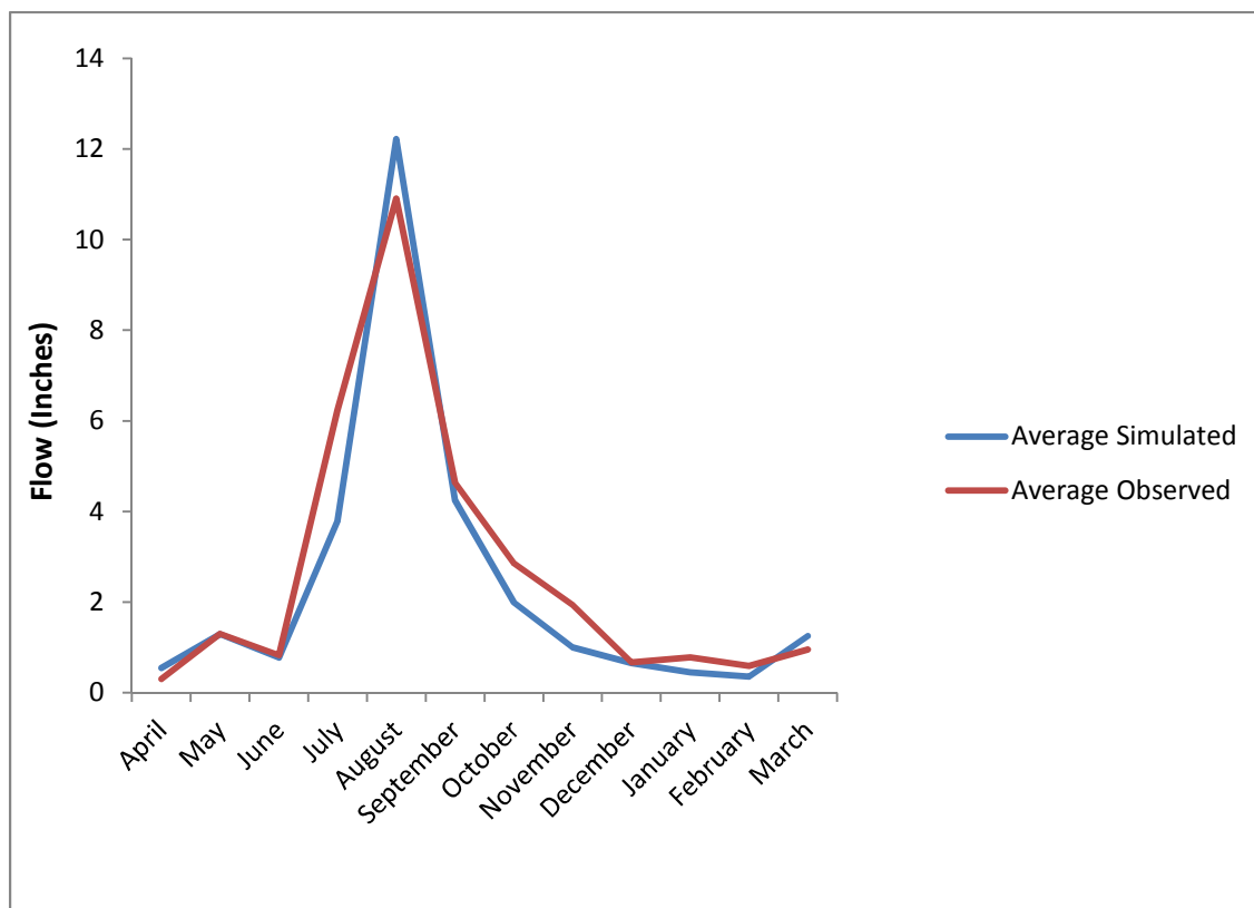
Fig6. Observed and Simulated Mean Monthly Streamflow for Paligad
