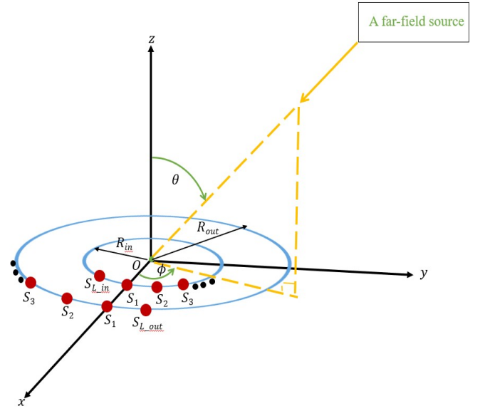
Fig. 2. A 2-circle concentric array.
