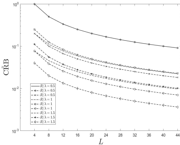
Fig. 5. CRB of (40), (41) and (42)
