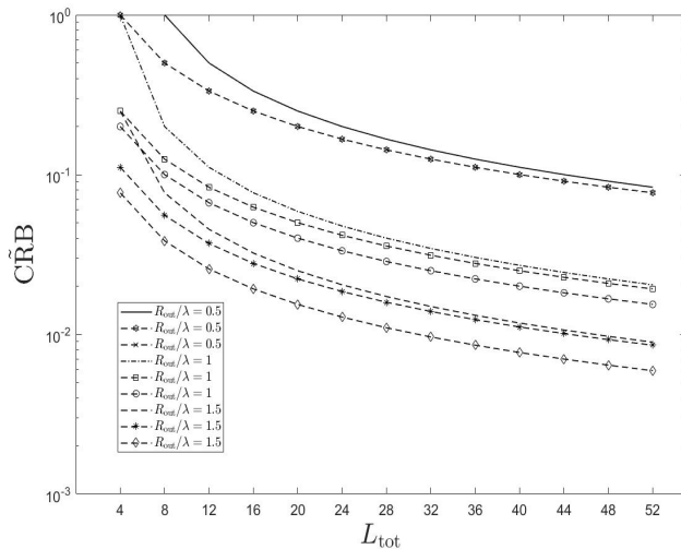
Fig. 6. CRB of (43), (44), and (45).
