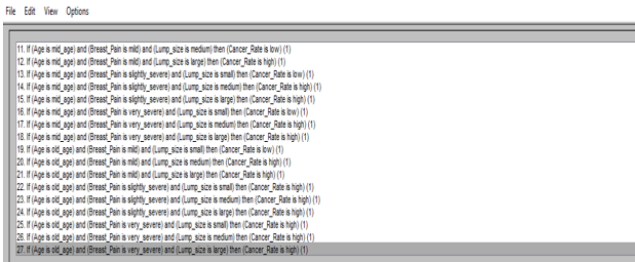
Figure 8: Screenshot of the fuzzy rules
