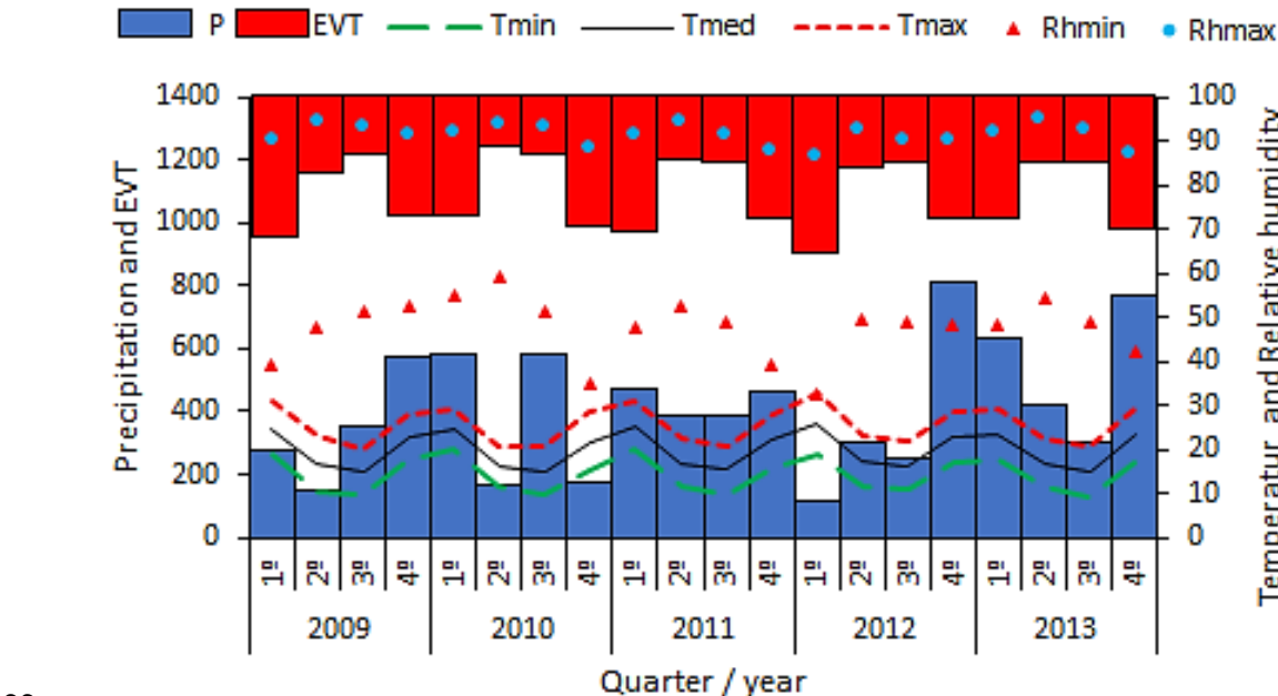
Figure 1: Meteorological diagram for the Alegrete region during tree growth.
