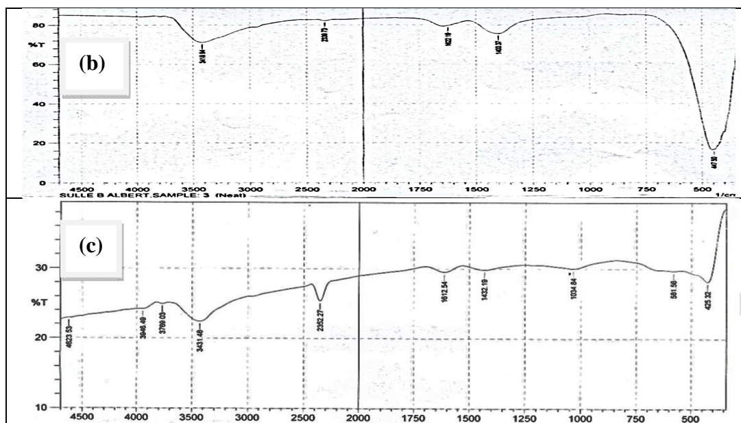
Fig.2. FTIR Spectra of (a) Powdered mixture of coconut shell and palm kernel shell (PCS+PPS), (b) Nano-sized nickel oxide filled activated carbon mixture of coconut shell and palm kernel shell (CS+PS) F and (c) Activated carbon mixture of coconut shell and palm kernel shell (CS+PS)
