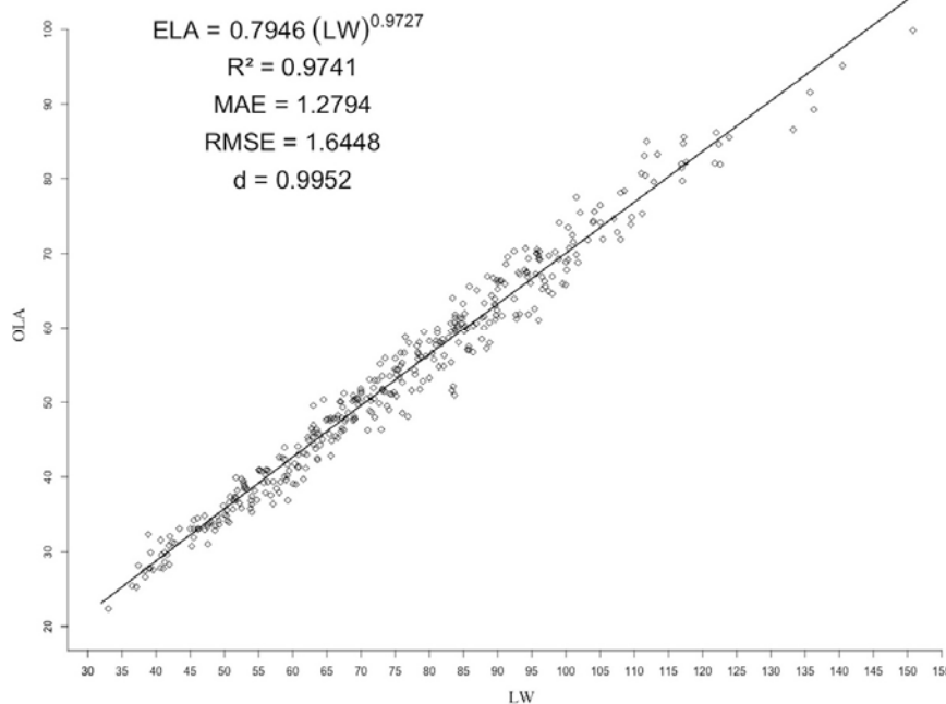
Figure 3. Equation of power model, determination coefficient ( R^2 ), the mean absolute error (MAE), the root mean square error (RMSE) and index d, using the foliar area observed
