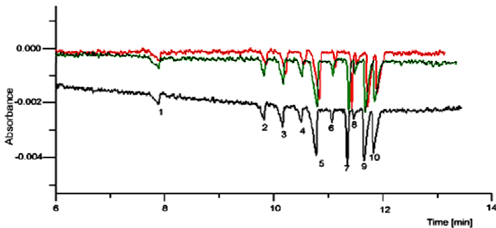
Fig.1b. The reproducibility (within runs) of metal ions over three runs using the same experimental conditions as in Fig. 1a. Peaks according to sequence: 1 = \text{K}^+ , 2 = \text{Ca}^{2+} , 3 = \text{Na}^+ , 4 = \text{Mg}^{2+} , 5 = \text{Mn}^{2+} , 6 = \text{Fe}^{2+} , 7 = \text{Cd}^{2+} , 8 = \text{Pb}^{2+} , 9 = \text{Ni}^{2+} , 10 = \text{Zn}^{2+} .
