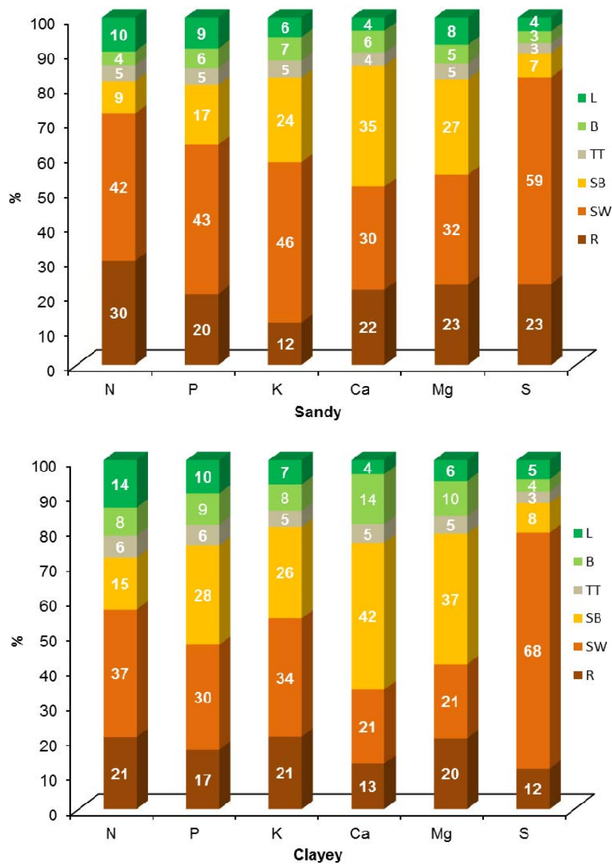
Figure 1. Distribution of nutrients in the different components of the biomass in a 7-years-old Eucalyptus urograndis stand, in the region of Telêmaco Borba, Parana - Brazil.
