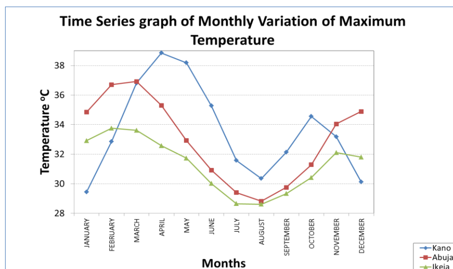
Figure 3: Monthly Variation of Maximum Temperature over selected cities
