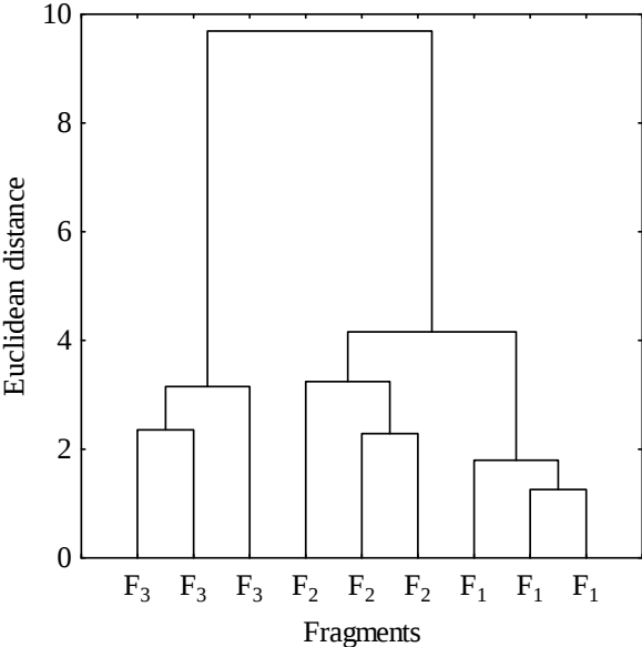
301 302 Figure 5. Dendrogram of dissimilarities between three forest fragments (F). 303 Jaboticabal, SP, 2015. 304
