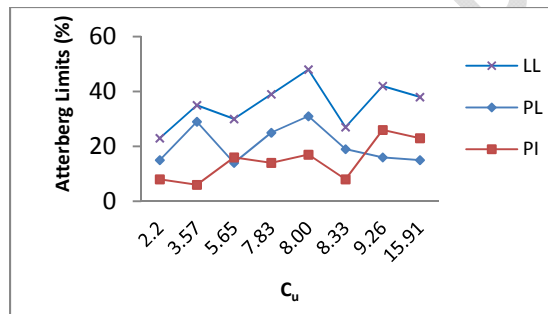
Figure 4: Relationship between Atterberg limits and coefficient of uniformity
