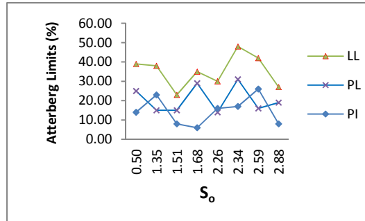
Figure 2: Relationship between Atterberg limits and sorting coefficient
