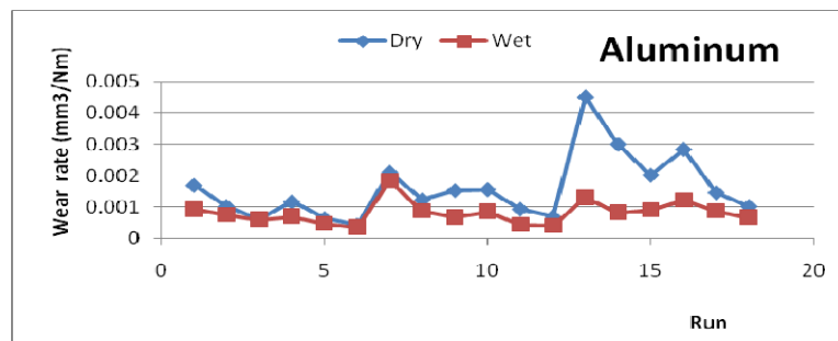
Fig. 2 Wear rate for Dry and Wet Conditions of Aluminium Sample
