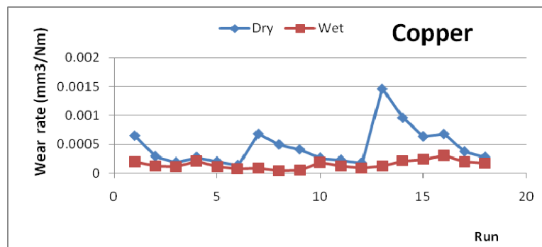
Fig. 3 Wear rate for Dry and Wet Conditions of Copper Sample
