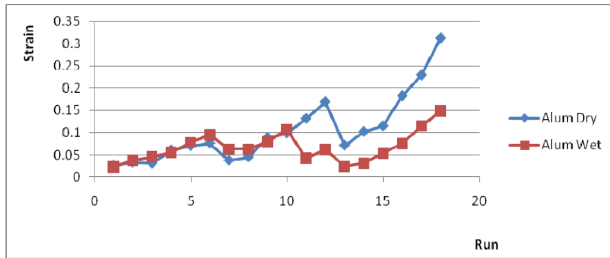
Fig. 10 Strain Deformation Curve on the Wear Track for Aluminium Sample
