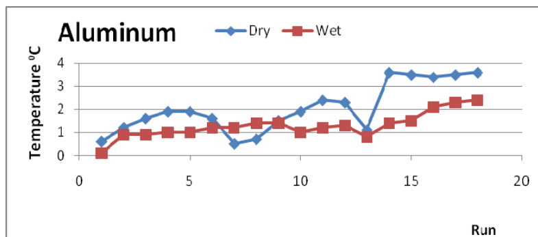
Fig. 5 Temperatures changes in Dry and Wet Aluminium with Number of run
