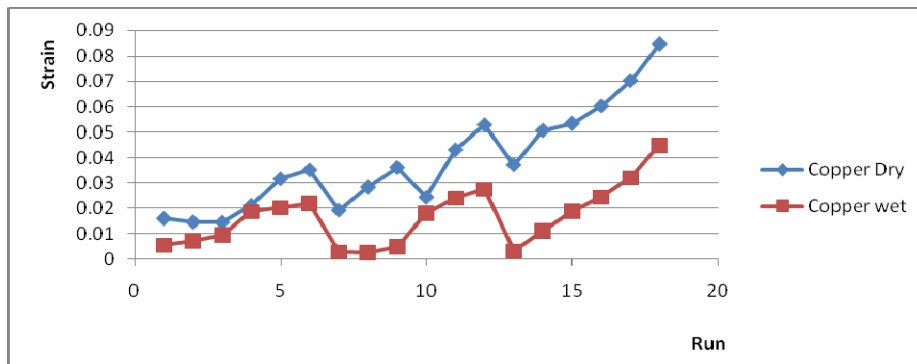
Fig. 11 Strain Deformation Curve on the Wear Track for the Copper Sample
