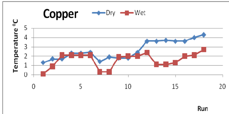
Fig. 6 Temperatures Changes in Dry and Wet Copper with Number of run
