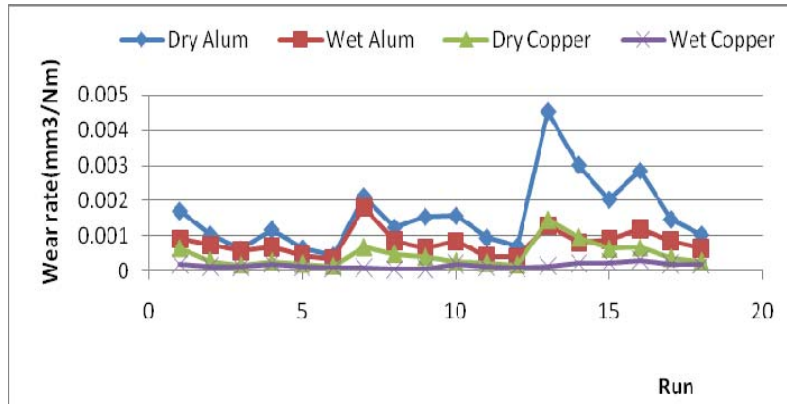
Fig. 4 Wear rate for Dry and Wet Conditions Comparison for Aluminium and Copper Samples
