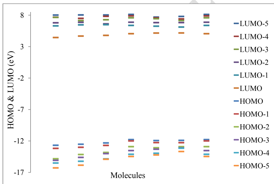
Figure8: HOMO and LUMO for antiperiplanar-molecules
