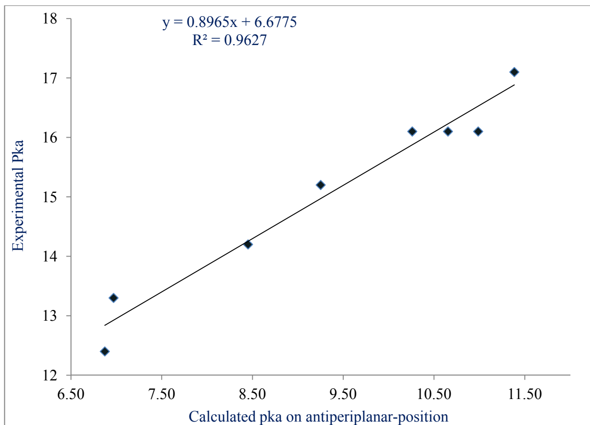
Figure2: the relationship between the calculated and experimental pKa in the antiperiplanar-position
