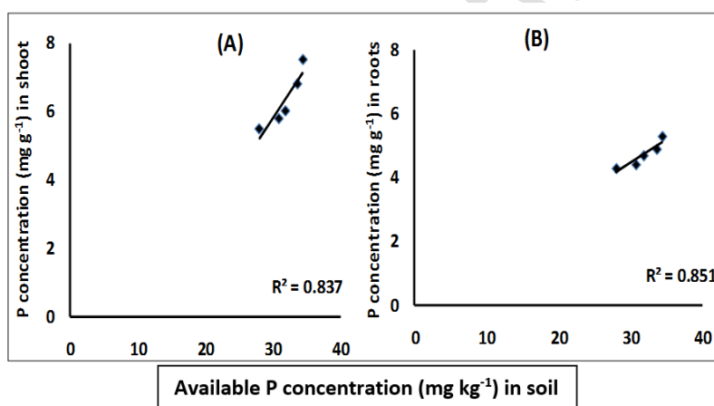
Fig. 3. The relationship between available P concentration in the studied soil and its concentration in shoots and roots of the growing wheat plants.
