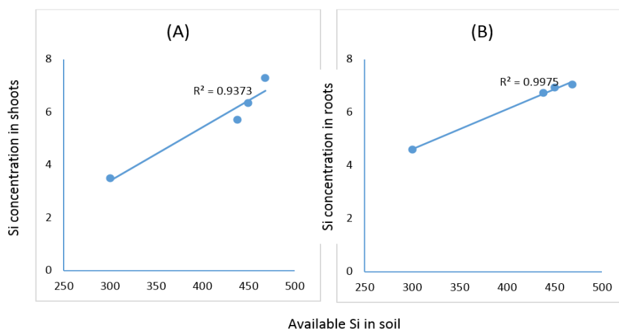
Fig. 2. The relationship between available Si concentration (mg kg -1 ) in the studied soil and its concentration (mg g -1 ) in shoots and roots of the growing wheat plants.
