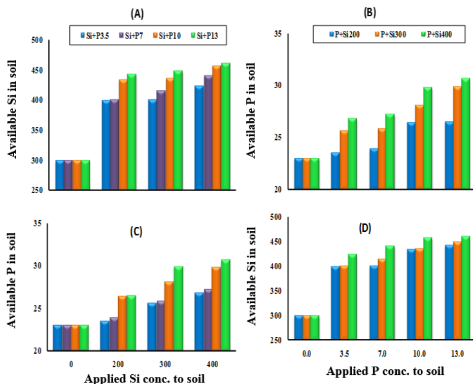
Fig 1. Available concentration (mg kg -1 ) of Si and P as affected by their interactions in the studied soil at booting growth stage of wheat plants.
