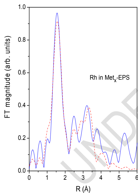
Fig. 6. Fourier transform magnitude of k_2 -weighted Rh K-edge EXAFS spectra of Rh in Met x -EPS sample, calculated in the k range 3–11 Å -1 and R range 1–3.4 Å. Experiment: solid line; best-fit EXAFS model of the nearest coordination shells: dashed line.
