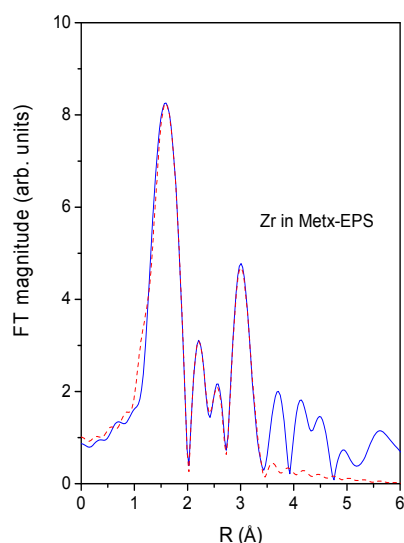
Fig. 5. Fourier transform magnitude of k_3 -weighted Zr K-edge EXAFS spectra of Zr in Met x -EPS sample, calculated in the k range 3–11 Å -1 and R range 1–3.4 Å. Experiment: solid line; best-fit EXAFS model of the nearest coordination shells: dashed line.
