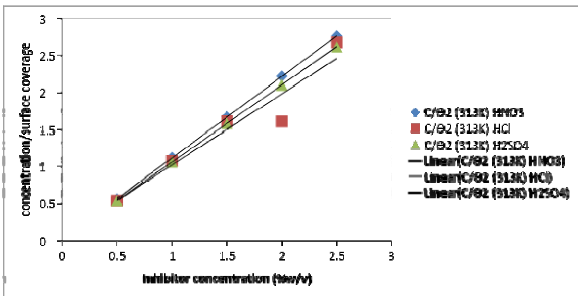
Fig.12. Langmuir isotherm plots of the corrosion of mild steel in 1M ( \text{HNO}_3 , \text{HCl} , \text{H}_2\text{SO}_4 ) in the presence of Azadirachta indica gum extract at 313K
