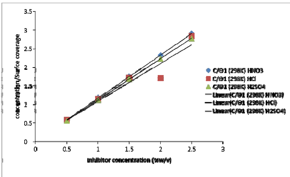
Fig.11. Langmuir isotherm plots of the corrosion of mild steel in 1M ( \text{HNO}_3 , \text{HCl} , \text{H}_2\text{SO}_4 ) in the presence of Azadirachta indica gum extract at 298K
