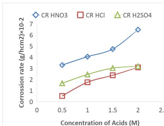
Fig.5. Variation of corrosion rate with concentration of the acids at 298K
