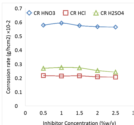
Fig.7 Variation of corrosion rate with concentration of the inhibitor at 298K.
