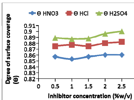
Fig. 10. The variations of surface coverage ( \theta ) with different inhibitor concentration at 313K are shown in below in the fig below:
