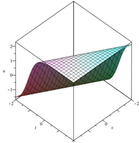
Figure 3.The plot of kink solution(4.2.7) When a_0 = 0.3, y = 0, z = 0
