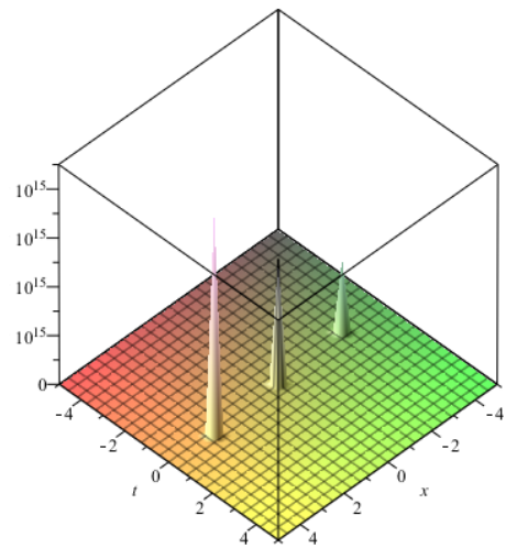
Figure 5.The plot of singular kink solution(4.3.6) When a_0 = -0.5, y = 0, z = 0
