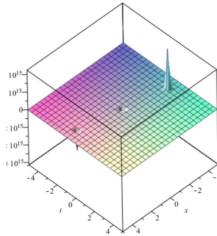
Figure 4.The plot of singular kink solution(4.2.8) when a_0 = -0.5, y = 0, z = 0
