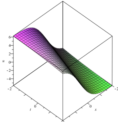
Figure 1. The plot of kink solution (4.1.7) When a_0 = 0.3, a = 1, y = 0, z = 0
