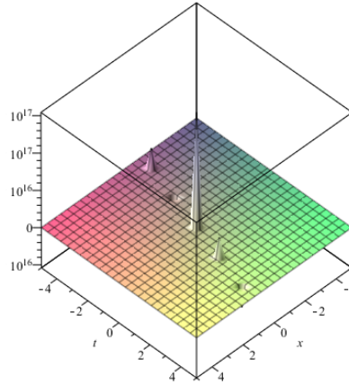
Figure 2. The plot of singular solution (4.1.9) when a_0 = 0.3, a = 1, y = 0, z = 0
