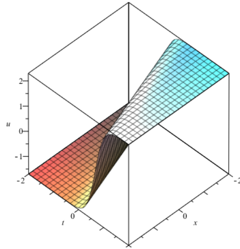
Figure 6.The plot of kink solution(4.3.9) when a_0 = 0.3, y = 0, z = 0
