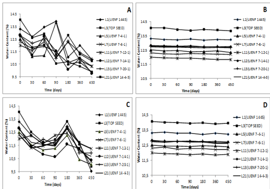
Figure 1. Variation of water content in the seeds of eight snap bean lines conditioned in different types of package and storage period (0, 30, 60, 90, 180, 360, and 450 days).(A) permeable package in an uncontrolled environment; (B) impermeable package in an uncontrolled environment; (C) permeable package in a cold chamber; (D) impermeable package in a cold chamber.
