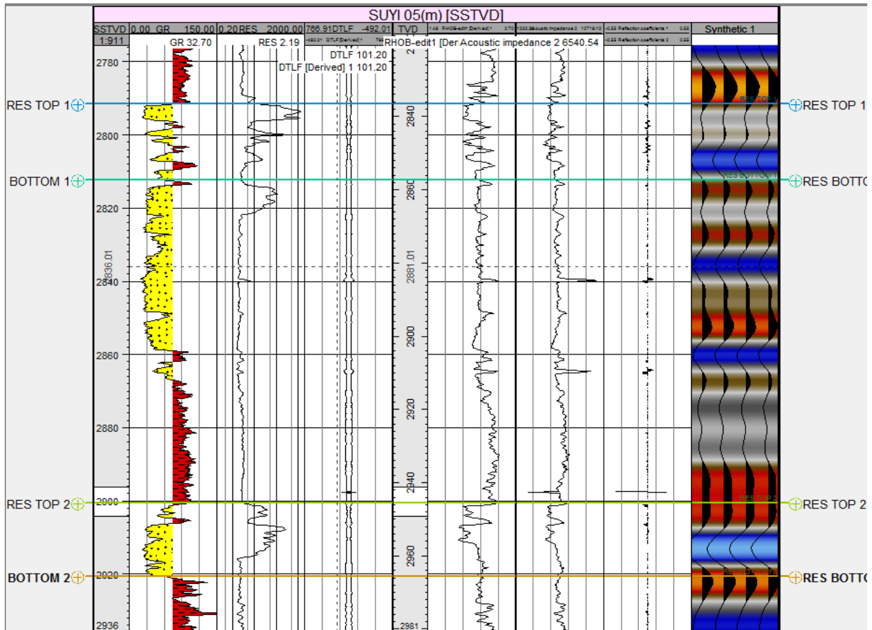
Fig. 4: SUIYI 05 Wells with Top and Base of Reservoir 1 and 2 respectively.
