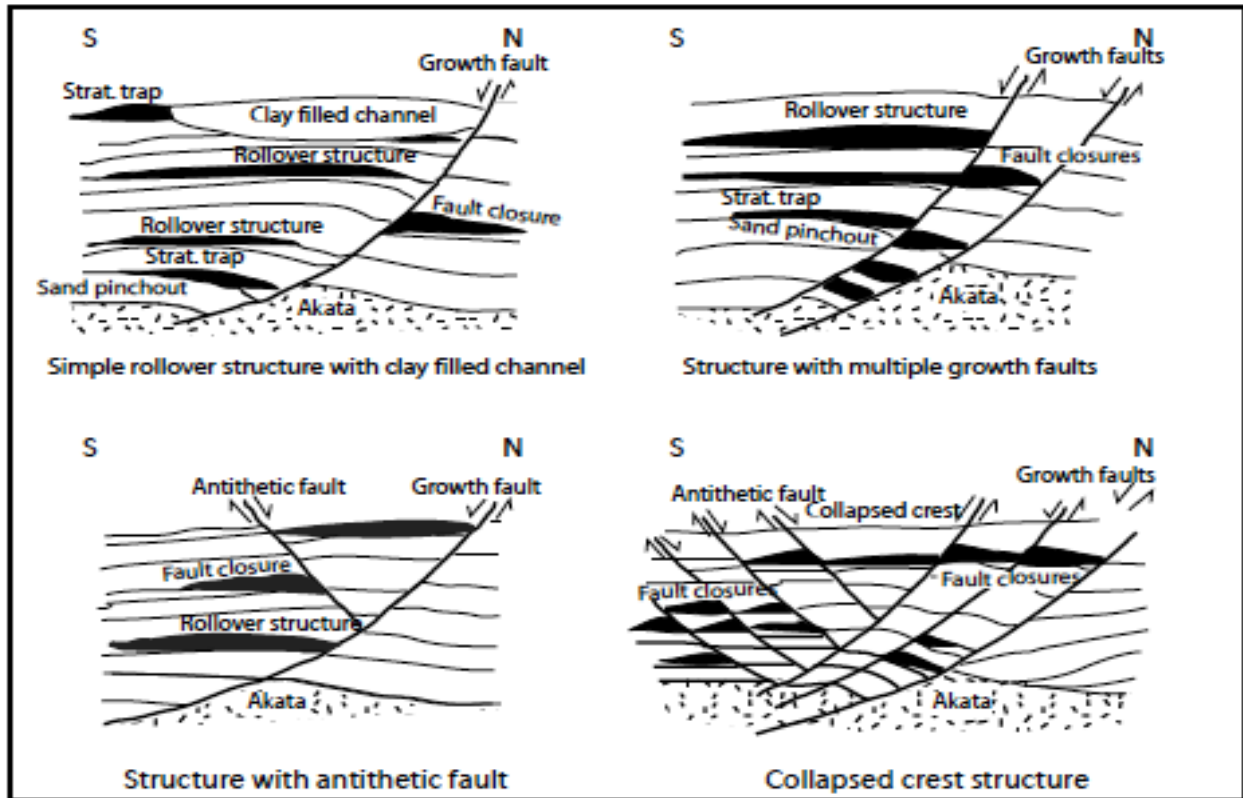
Fig. 3: Examples of Niger Delta oil field structures and associated trap types. Modified from {6, 10 and 16}.
