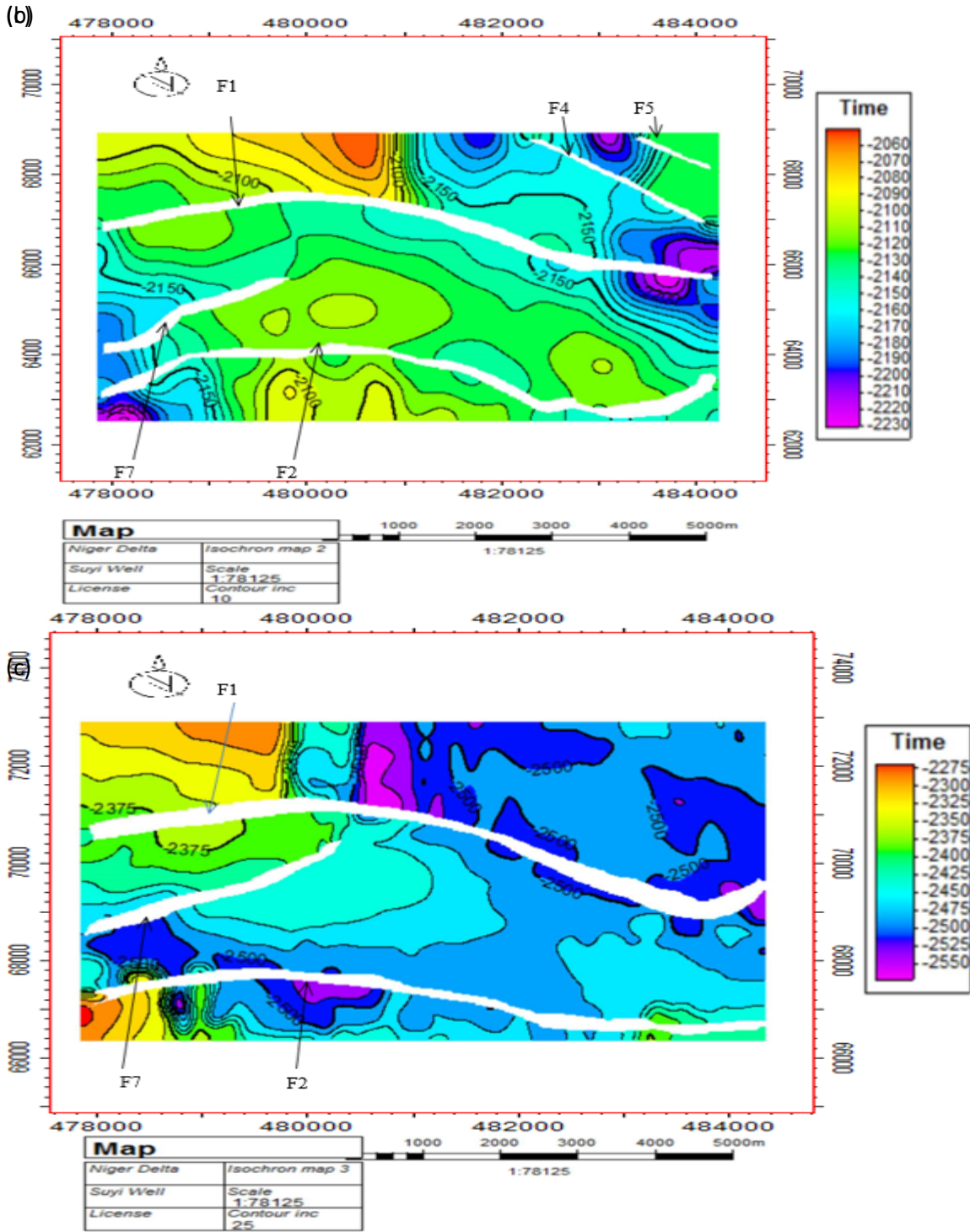
Fig. 6: a, b and c: Time structure map of Horizon 1, 2 and 3 respectively.
