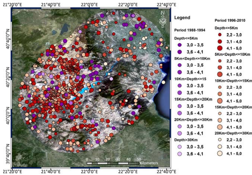
Fig. 4. Spatial distribution map for the period 1988-1994 and 1996-2010.
