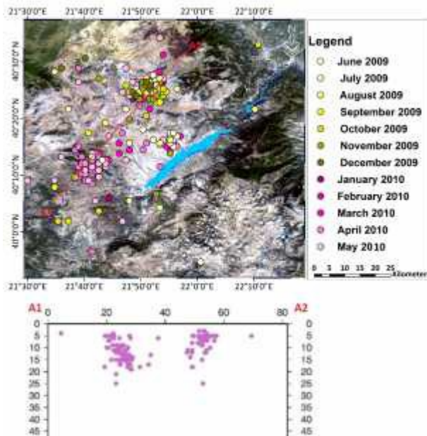
Fig. 5. Evolution of the seismicity in the study area during the period June 2009 – May 2010 ( 2.5 < M_L \leq 3.7 ) and the cross section A_1A_2 (strike 30^\circ ).
