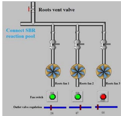
Fig. 9 Blower room
