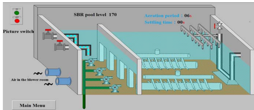
Fig.8 SBR pool
