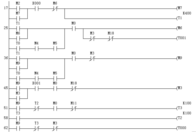
Fig.10 Grille, gathering pool ladder diagram
