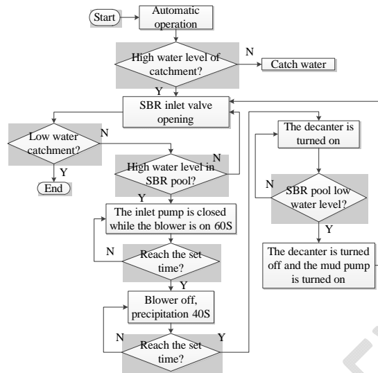
Fig.11 SBR reaction pool program design flow chart
