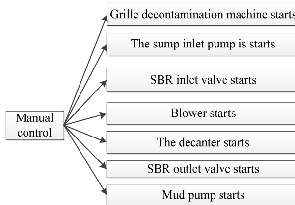
Fig.6 Manual mode control chart
