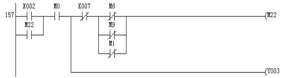
Fig.13 Ladder diagram of inlet condition for SBR reaction tank 2
