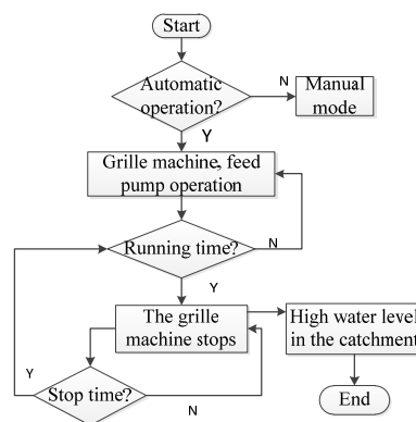
Fig.8 Grid design flow chart
