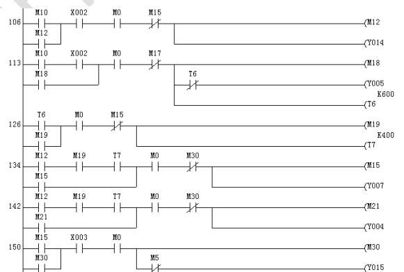
Fig.12 SBR pool flow ladder diagram
