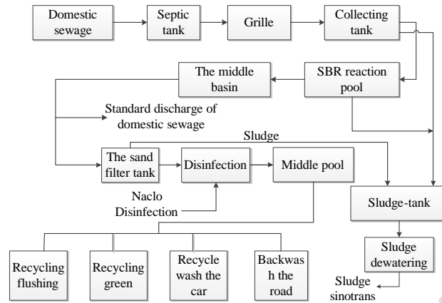
Fig.3 System process flow chart
