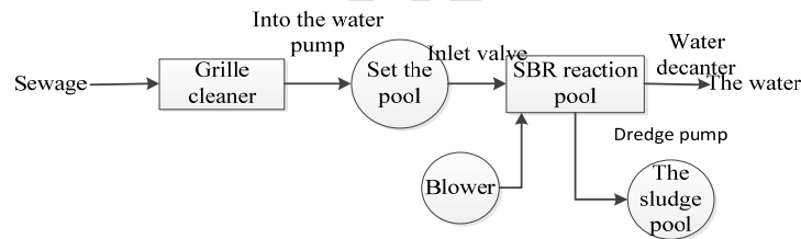
Fig.7 Automatic mode control flow chart
