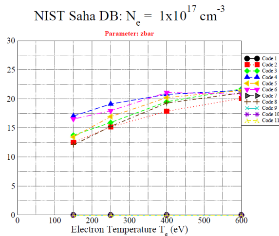
Figure 4.a. Germanium plasma properties computed with codes of NLTE-3 Workshop
