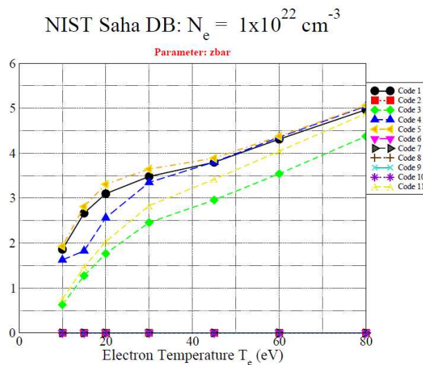
Figure 1.a. Carbon plasma properties computed with codes of NLTE-3 Workshop
