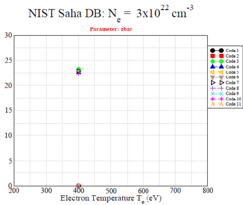
Figure 4.c. Germanium plasma properties computed with codes of NLTE-3 Workshop
