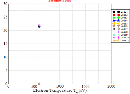
Figure 4.b. Germanium plasma properties computed with codes of NLTE-3 Workshop
