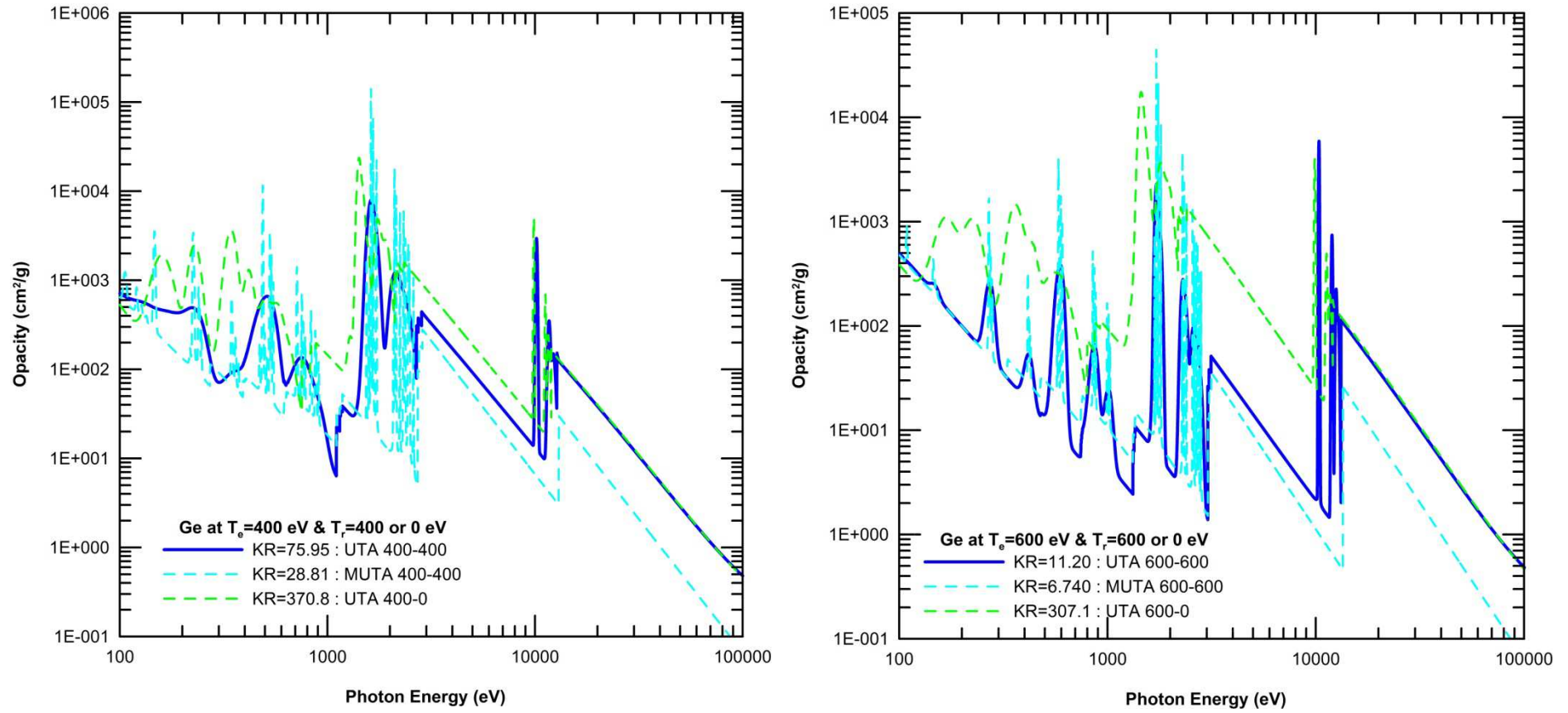
Figure 4.e. Frequency resolved opacity of germanium plasma at density 3E+22 \text{cm}^{-3} with ATMED CR at T_{\text{rad}} = 400 eV in UTA (—) or MUTA (- -) formalisms or T_{\text{rad}} = 0 eV in UTA (- · -) formalism and T_e = 400 eV observing the sensitivity to departures from LTE regime (left). Germanium plasma frequency resolved opacity of ATMED CR at T_{\text{rad}} = 600 eV in UTA (—) or MUTA (- -) formalisms or T_{\text{rad}} = 0 eV in UTA (- · -) formalism and T_e = 600 eV observing the sensitivity to departures from LTE regime (right).
