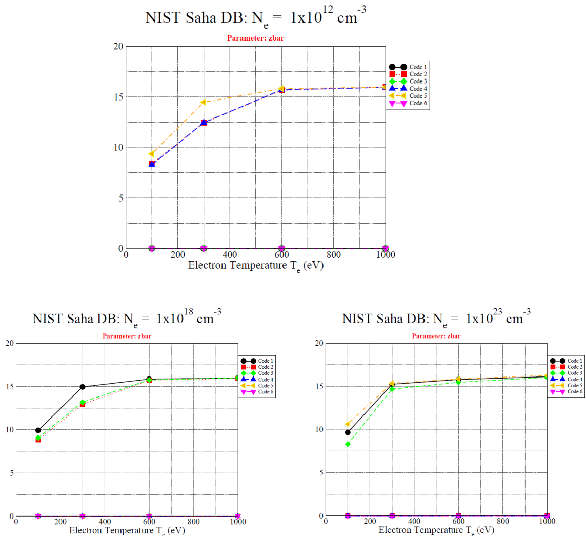
Figure 3.a. Argon plasma properties computed with codes of NLTE-3 Workshop
