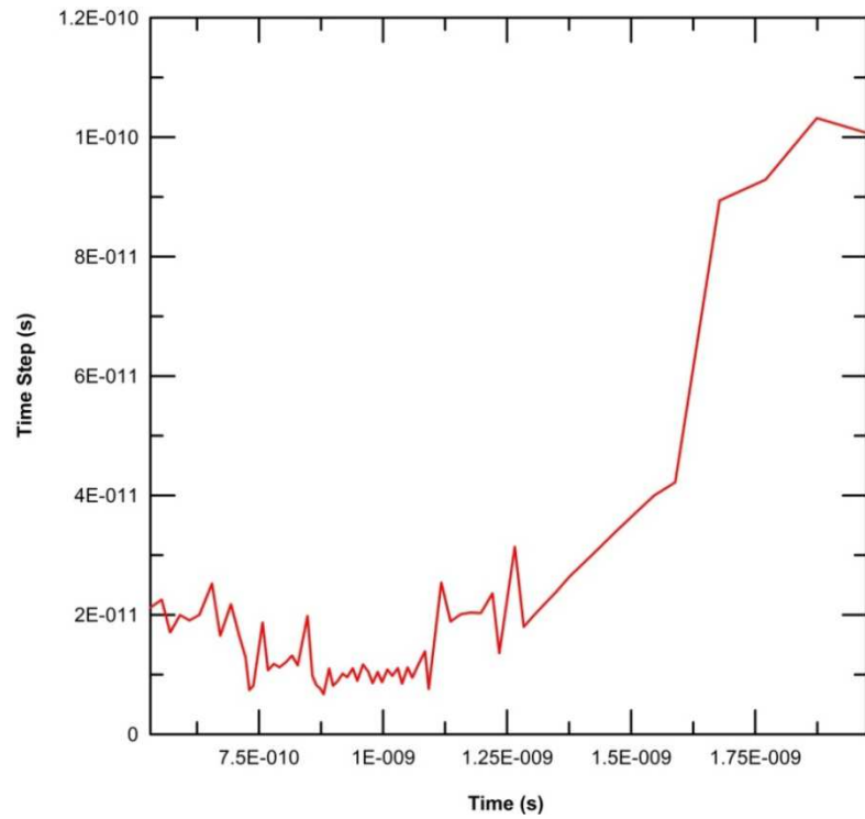
Figure 7.b. Time step evolution of plasma case TD-Ge provided by Workshop NLTE-3 (left). Temporal mean charge of germanium plasma computed with ATMED CR (right), with criteria of convergence in populations of < 1E-02, < 1.5E-02 or more strict < 5E-04.
