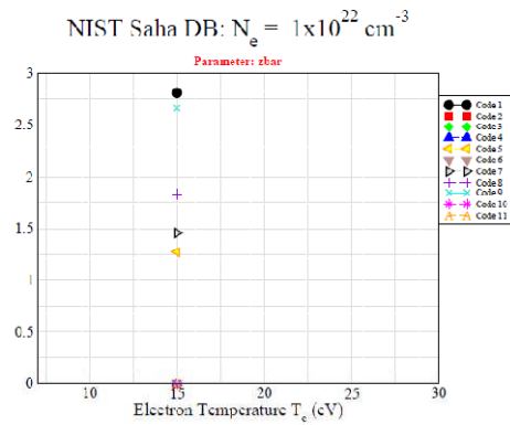
Figure 1.b. Carbon plasma properties computed with codes of NLTE-3 Workshop
