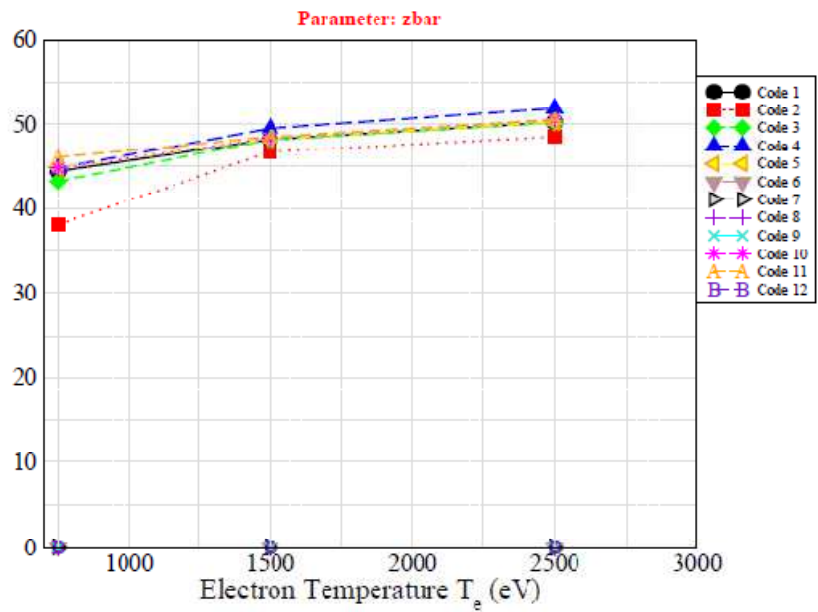
Figure 6.b. Gold plasma properties computed with codes of NLTE-3 Workshop
