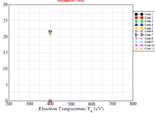
Figure 4.b. Germanium plasma properties computed with codes of NLTE-3 Workshop
