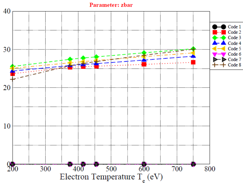
Figure 5.b. Xenon plasma properties computed with codes of NLTE-3 Workshop
