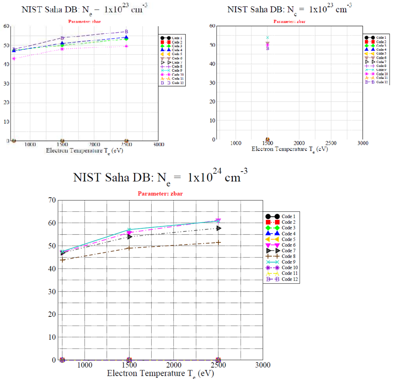
Figure 6.c. Gold plasma properties computed with codes of NLTE-3 Workshop
