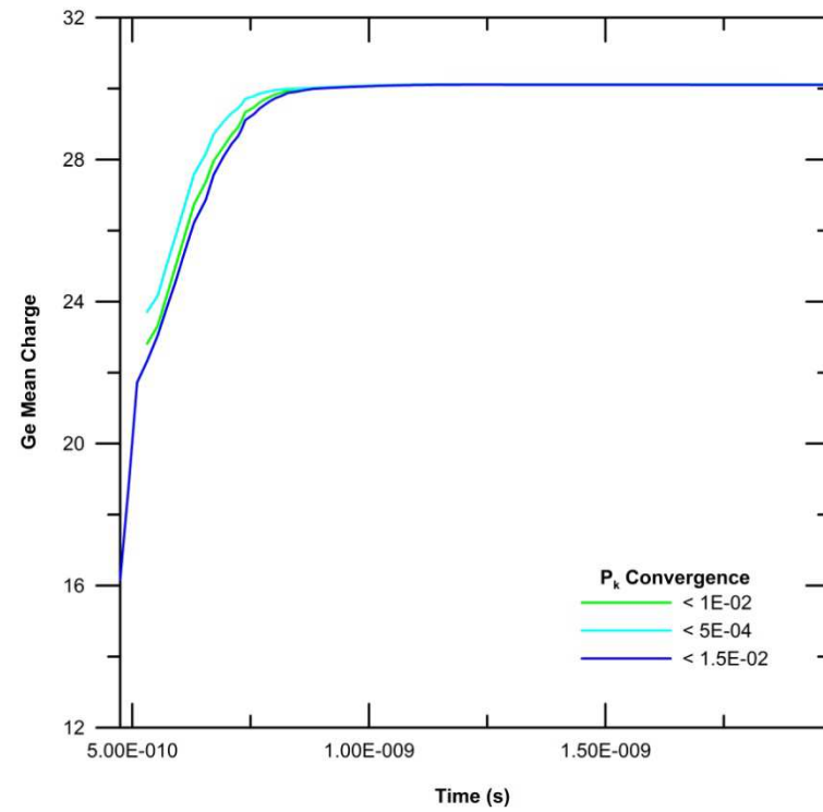
Figure 7.b. Time step evolution of plasma case TD-Ge provided by Workshop NLTE-3 (left). Temporal mean charge of germanium plasma computed with ATMED CR (right), with criteria of convergence in populations of < 1E-02, < 1.5E-02 or more strict < 5E-04.
