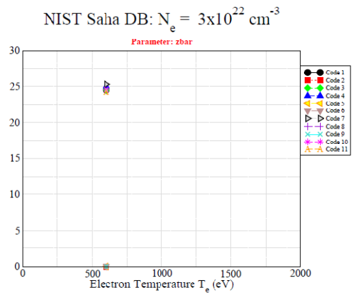
Figure 4.c. Germanium plasma properties computed with codes of NLTE-3 Workshop
