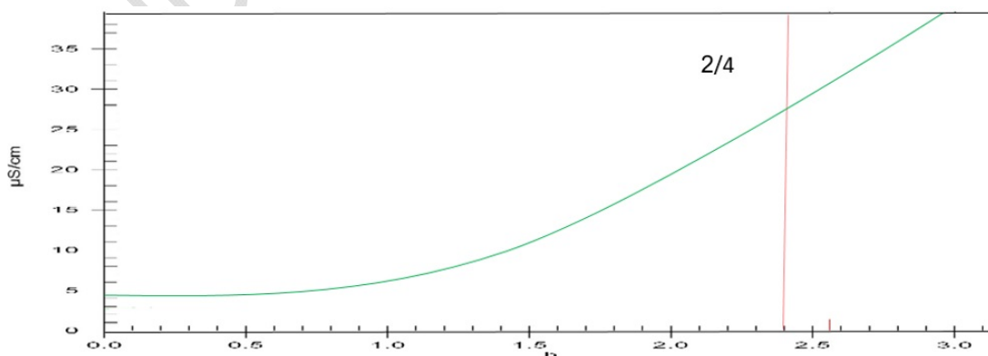
Fig 2: Rancimat test for treatment contained 5% of BCO
