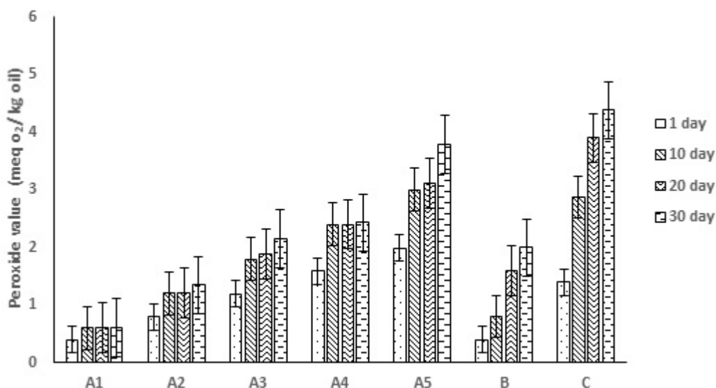
Fig 3: Changes in Peroxide value (PV) of treated Flaxseed oil samples at different storage time (1, 10, 20 and 30 th days)
