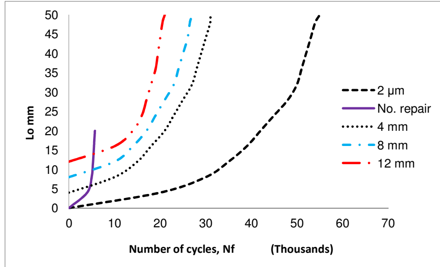
Fig.9: Fatigue crack growth curves of beams strengthened at different notch (crack) length
