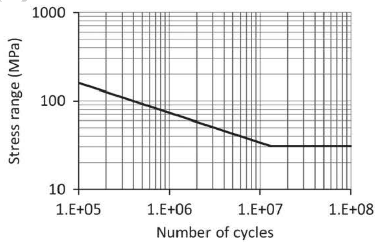
Fig.4: S-N curve of steel beams
