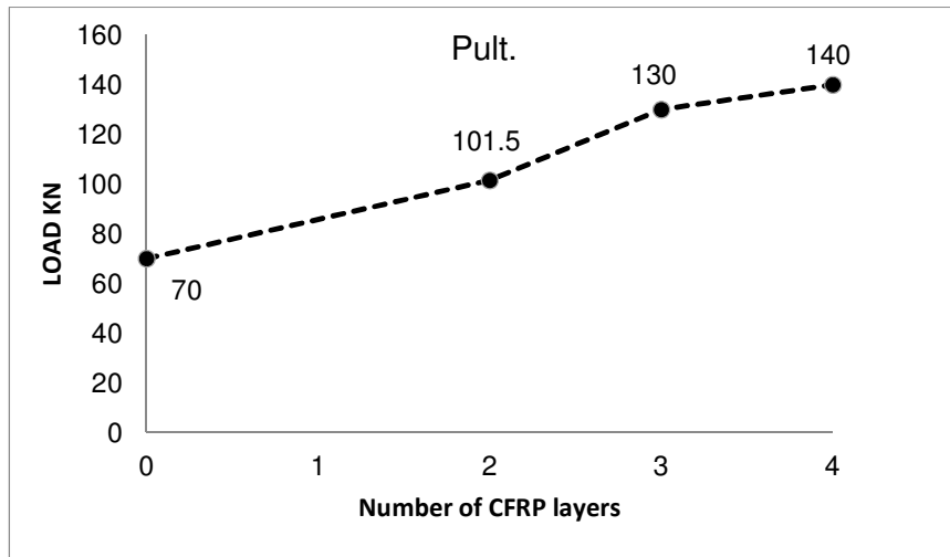
Fig.7: Effect of number of CFRP layers on ultimate load
