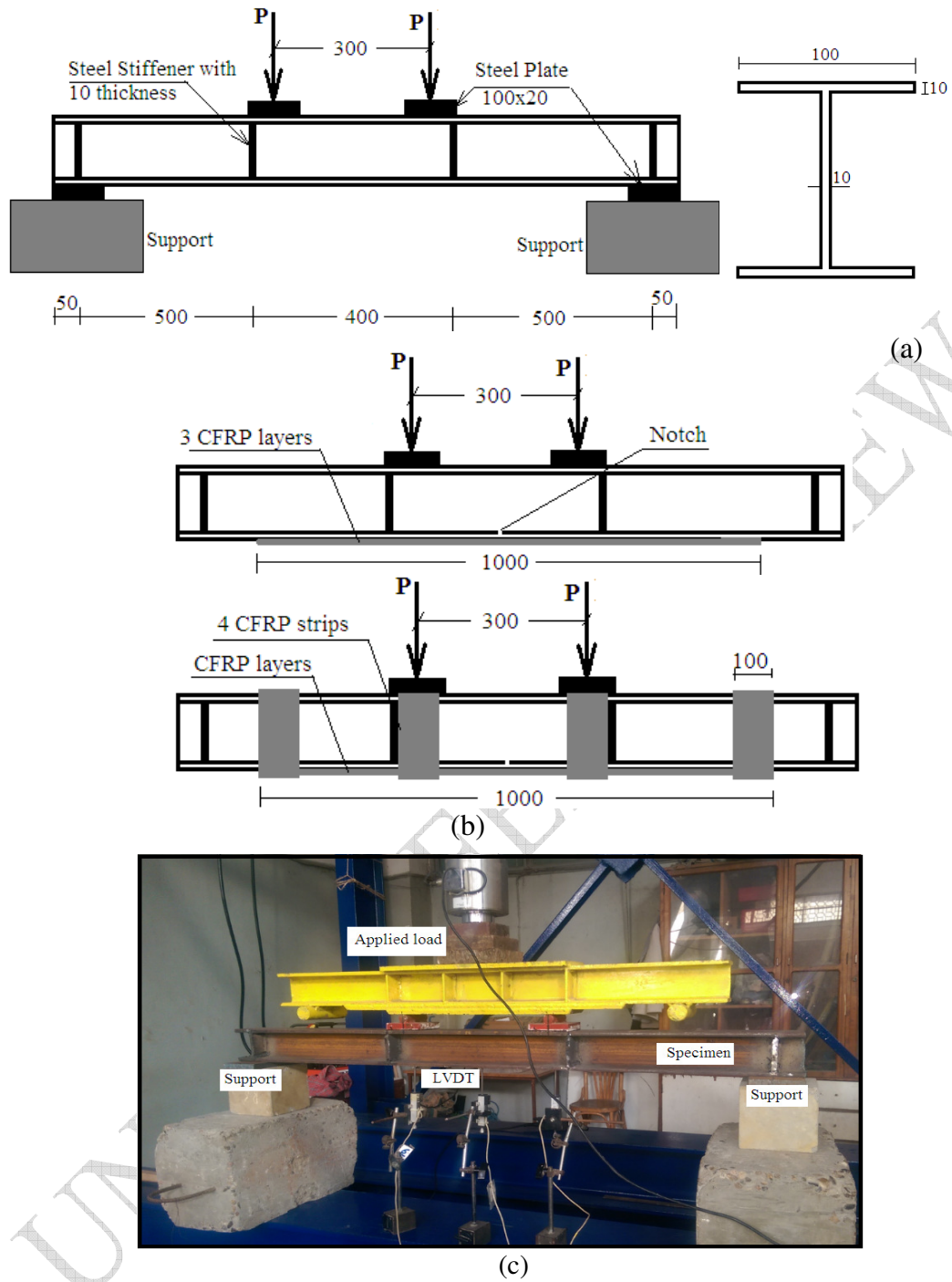
Fig. 1: Experimental test (a) specimen geometry "dimension in millimeter, not to scale", (b) details of the strengthened beams and notch details, (c) test set-up details
