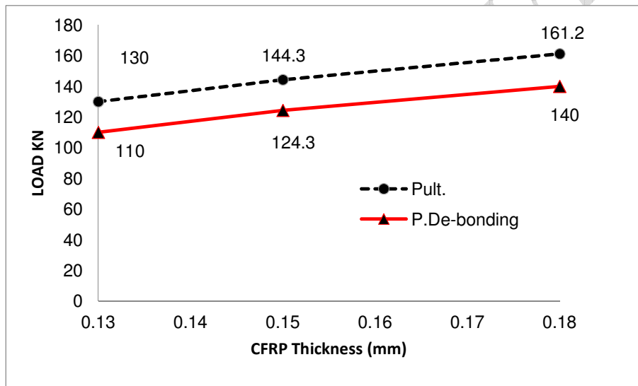
Fig.8: Effect of CFRP thickness on ultimate and de-bonding loads
