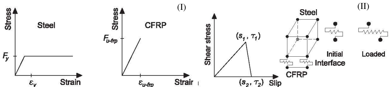
Fig. 2: Material modeling (I) Constitutive behavior of Steel and CFRP, (II) Interface element model
