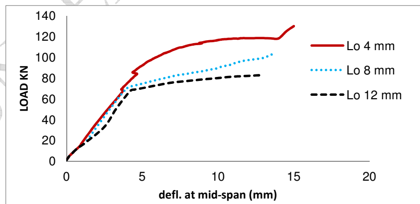
Fig.6: Load – deflection curve strengthened beam with different notch length (Lo)
