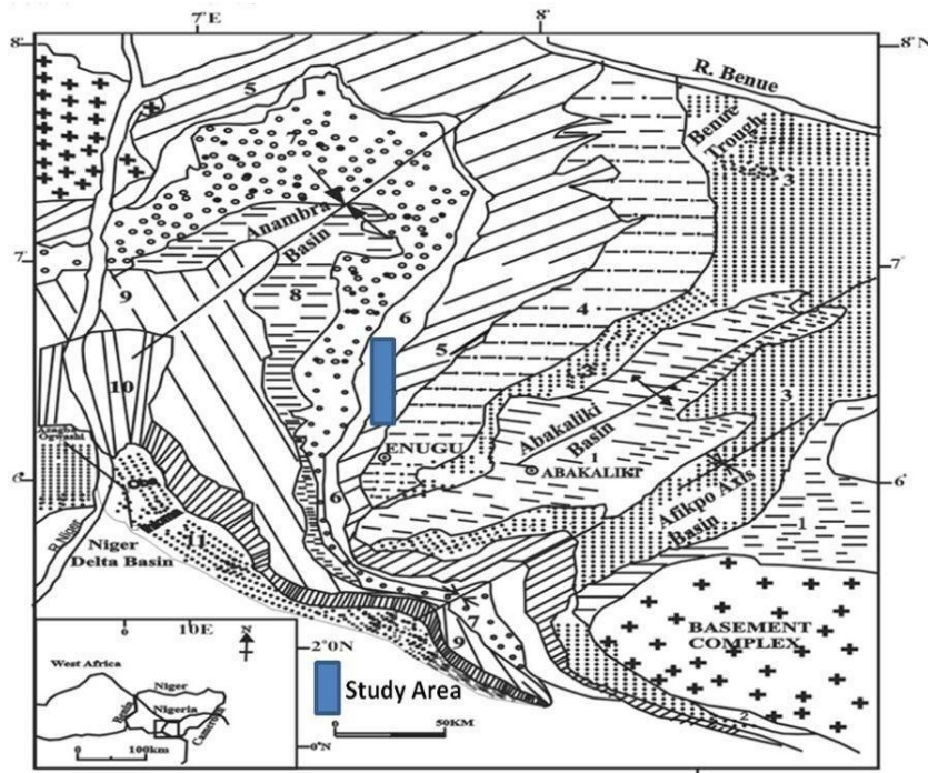
Fig. 1. Geologic Map of Anambra Basin and Afikpo Basin South-Eastern Nigeria showing the study area: 1. Asu River Group; 2. Odukpani Formation; 3. Ezeaku Shale; 4. Awgu Shale; 5. Enugu/Nkporo Shale; 6. Mamu Formation; 7. Ajali Sandstone; 8. Nsukka Formation; 9. Imo Shale; 10. Ameki Formation; 11. Ogwashi Asaba Formation. Source: Chiagbanam et al 10 .
